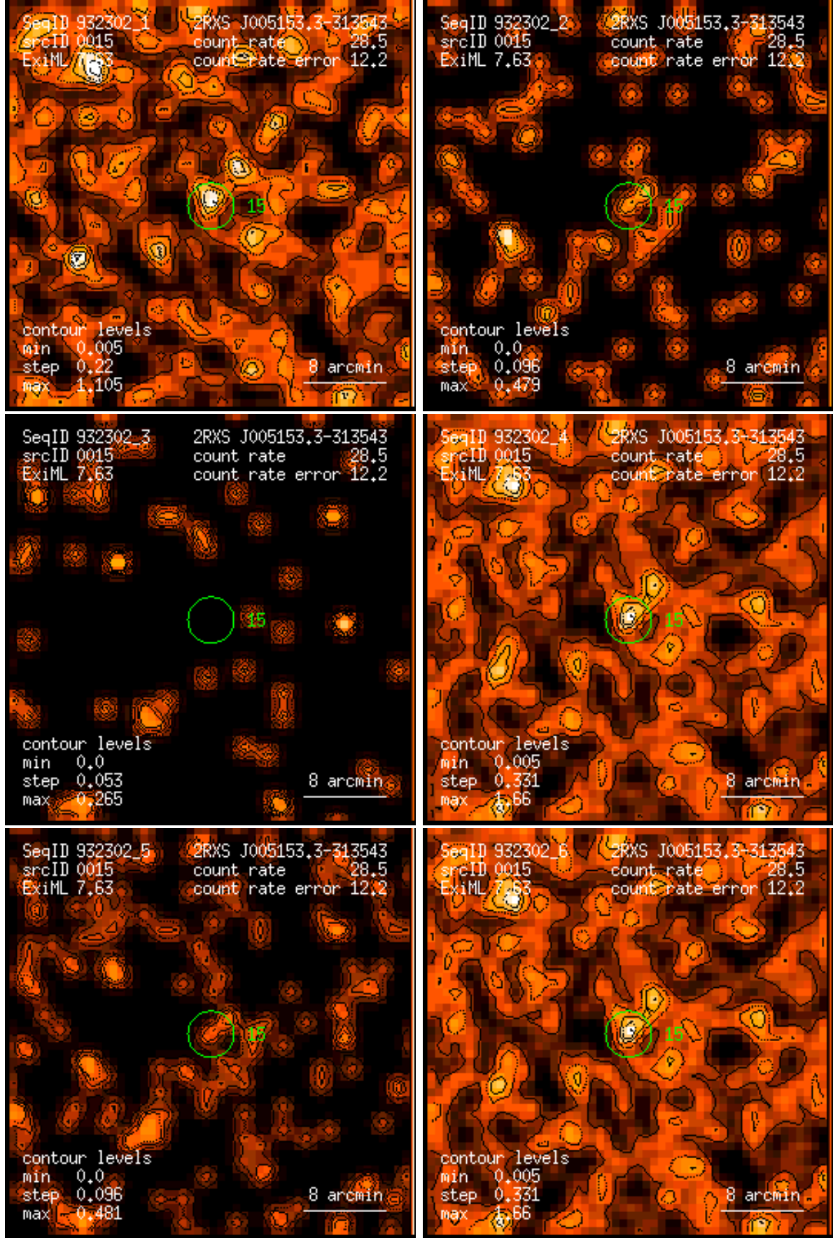
Figure 15: RASS 932302: detection 0015: band rate images, Gaussian filter: (1) PSPC channels 11 – 41, (2) 52 – 90, (3) 91 – 201, (4) 11 – 235, (5) 52 – 201, (6) 11 – 201. Broad band rates in counts/ks. Band rate contour levels in counts/ks/arcmin 2 .
