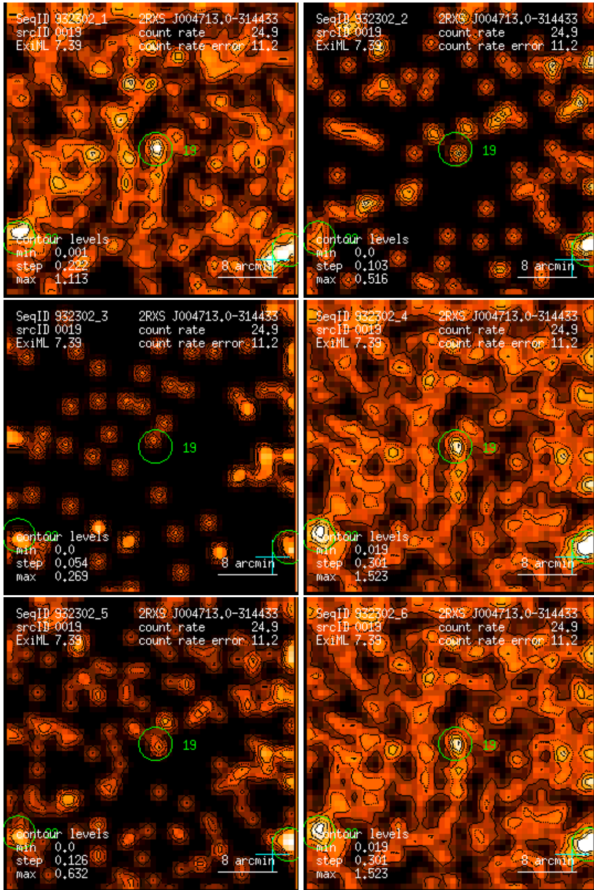
Figure 19: RASS 932302: detection 0019: band rate images, Gaussian filter: (1) PSPC channels 11 – 41, (2) 52 – 90, (3) 91 – 201, (4) 11 – 235, (5) 52 – 201, (6) 11 – 201. Broad band rates in counts/ks. Band rate contour levels in counts/ks/arcmin 2 .
