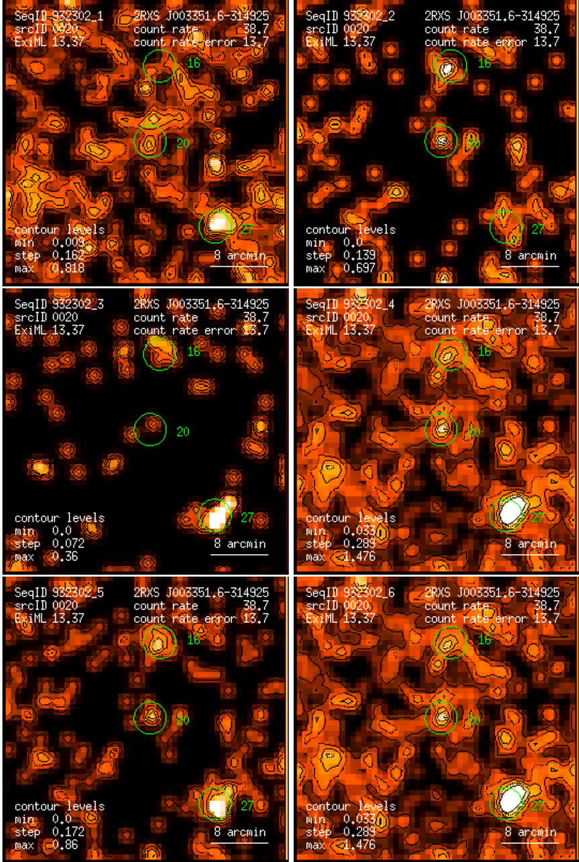
Figure 20: RASS 932302: detection 0020: band rate images, Gaussian filter: (1) PSPC channels 11 – 41, (2) 52 – 90, (3) 91 – 201, (4) 11 – 235, (5) 52 – 201, (6) 11 – 201. Broad band rates in counts/ks. Band rate contour levels in counts/ks/arcmin 2 .
