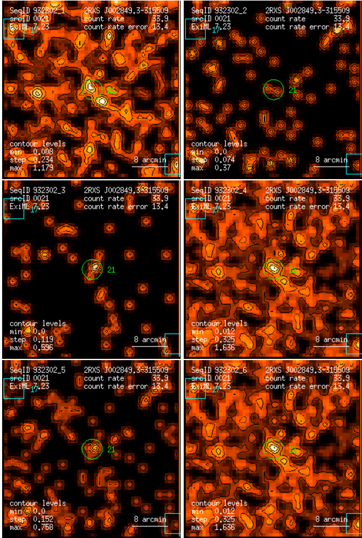
Figure 21: RASS 932302: detection 0021: band rate images, Gaussian filter: (1) PSPC channels 11 – 41, (2) 52 – 90, (3) 91 – 201, (4) 11 – 235, (5) 52 – 201, (6) 11 – 201. Broad band rates in counts/ks. Band rate contour levels in counts/ks/arcmin 2 .
