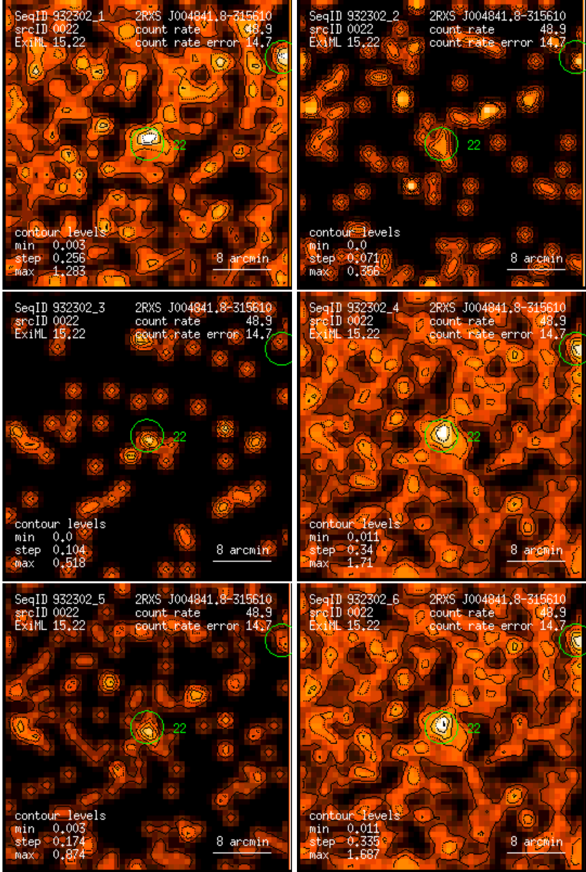
Figure 22: RASS 932302: detection 0022: band rate images, Gaussian filter: (1) PSPC channels 11 – 41, (2) 52 – 90, (3) 91 – 201, (4) 11 – 235, (5) 52 – 201, (6) 11 – 201. Broad band rates in counts/ks. Band rate contour levels in counts/ks/arcmin 2 .
