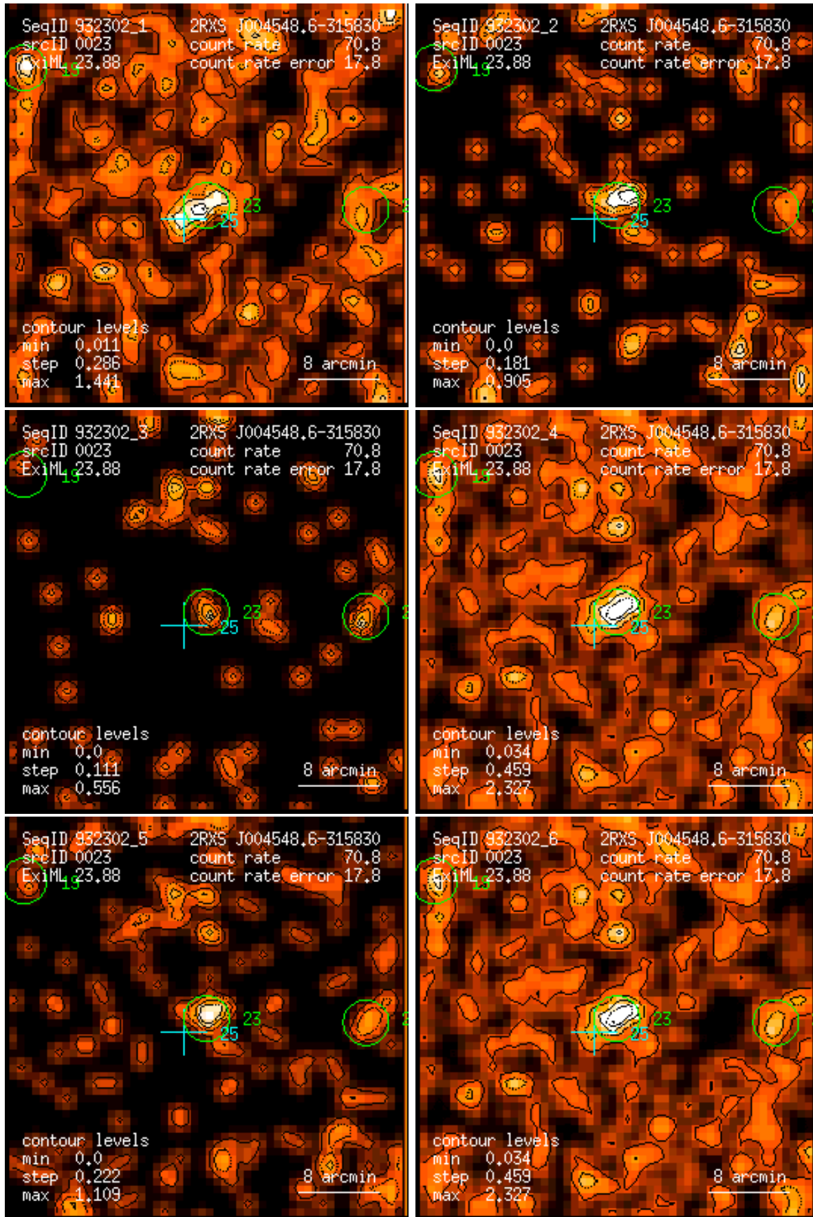
Figure 23: RASS 932302: detection 0023: band rate images, Gaussian filter: (1) PSPC channels 11 – 41, (2) 52 – 90, (3) 91 – 201, (4) 11 – 235, (5) 52 – 201, (6) 11 – 201. Broad band rates in counts/ks. Band rate contour levels in counts/ks/arcmin 2 .
