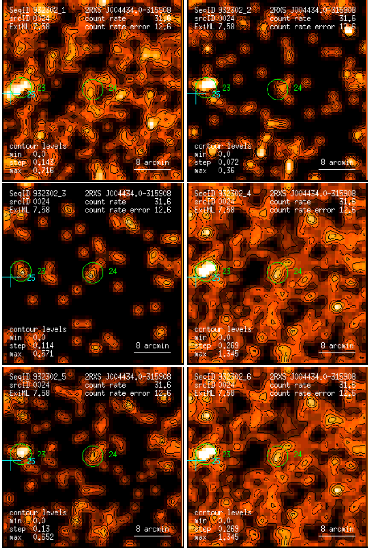
Figure 24: RASS 932302: detection 0024: band rate images, Gaussian filter: (1) PSPC channels 11 – 41, (2) 52 – 90, (3) 91 – 201, (4) 11 – 235, (5) 52 – 201, (6) 11 – 201. Broad band rates in counts/ks. Band rate contour levels in counts/ks/arcmin 2 .
