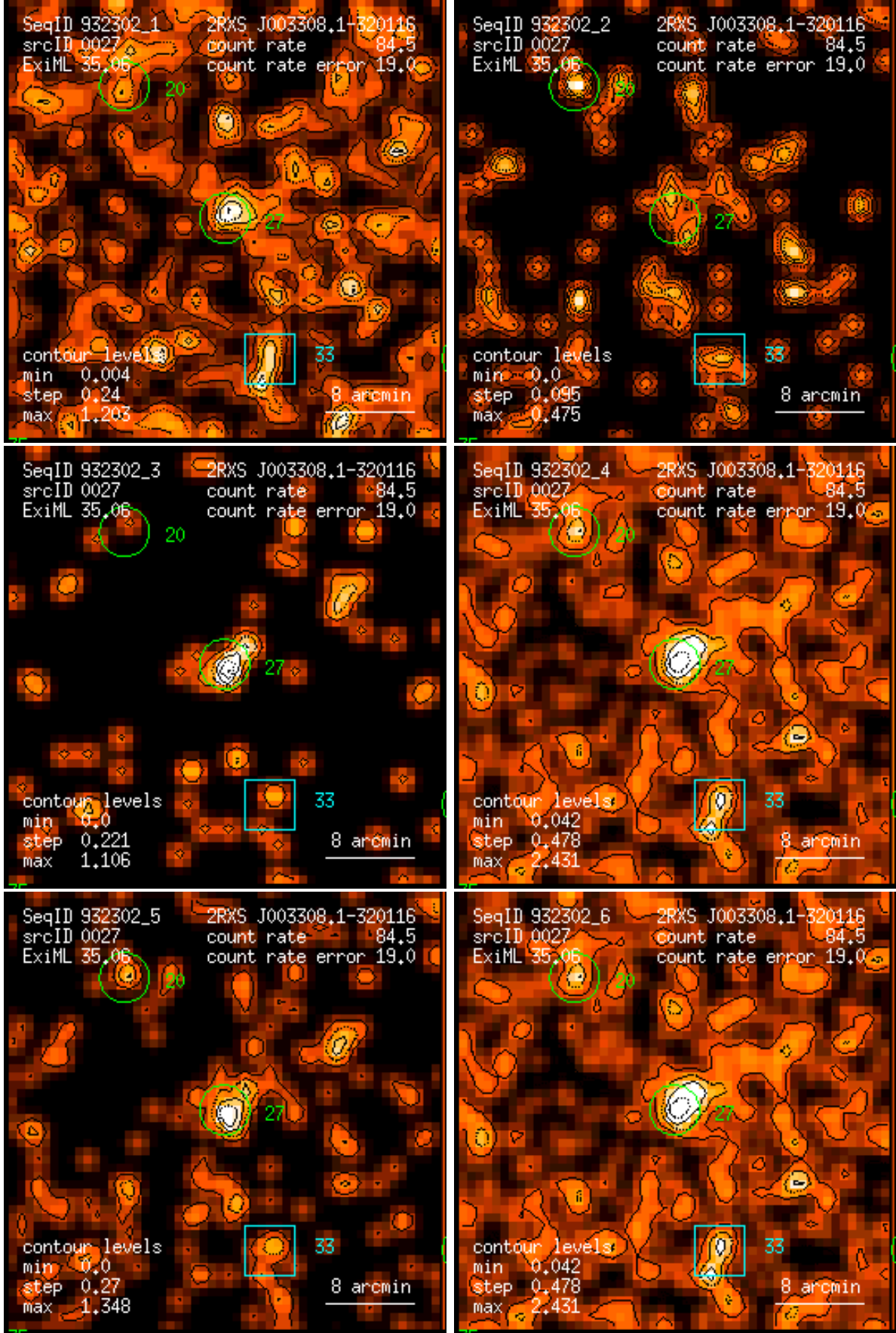
Figure 27: RASS 932302: detection 0027: band rate images, Gaussian filter: (1) PSPC channels 11 – 41, (2) 52 – 90, (3) 91 – 201, (4) 11 – 235, (5) 52 – 201, (6) 11 – 201. Broad band rates in counts/ks. Band rate contour levels in counts/ks/arcmin 2 .
