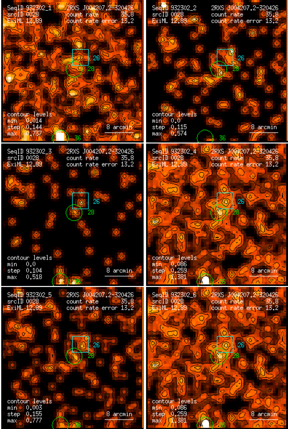
Figure 28: RASS 932302: detection 0028: band rate images, Gaussian filter: (1) PSPC channels 11 – 41, (2) 52 – 90, (3) 91 – 201, (4) 11 – 235, (5) 52 – 201, (6) 11 – 201. Broad band rates in counts/ks. Band rate contour levels in counts/ks/arcmin 2 .
