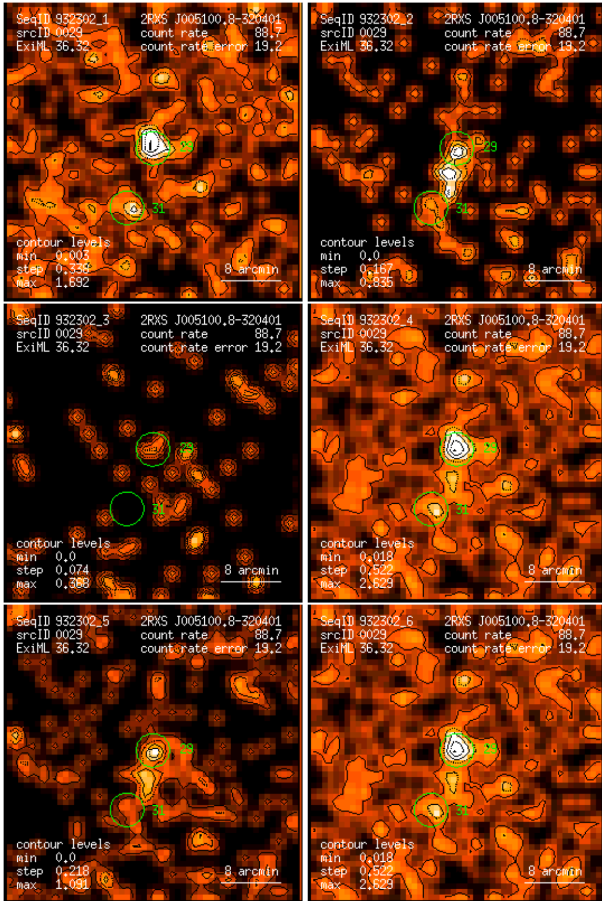
Figure 29: RASS 932302: detection 0029: band rate images, Gaussian filter: (1) PSPC channels 11 – 41, (2) 52 – 90, (3) 91 – 201, (4) 11 – 235, (5) 52 – 201, (6) 11 – 201. Broad band rates in counts/ks. Band rate contour levels in counts/ks/arcmin 2 .
