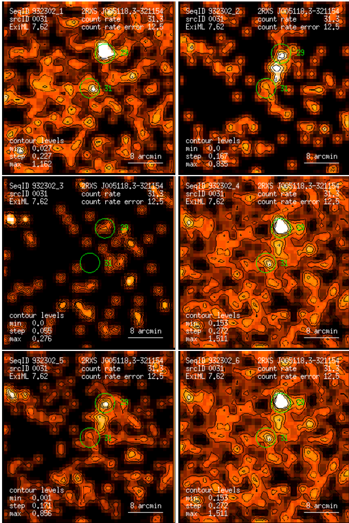
Figure 31: RASS 932302: detection 0031: band rate images, Gaussian filter: (1) PSPC channels 11 – 41, (2) 52 – 90, (3) 91 – 201, (4) 11 – 235, (5) 52 – 201, (6) 11 – 201. Broad band rates in counts/ks. Band rate contour levels in counts/ks/arcmin 2 .
