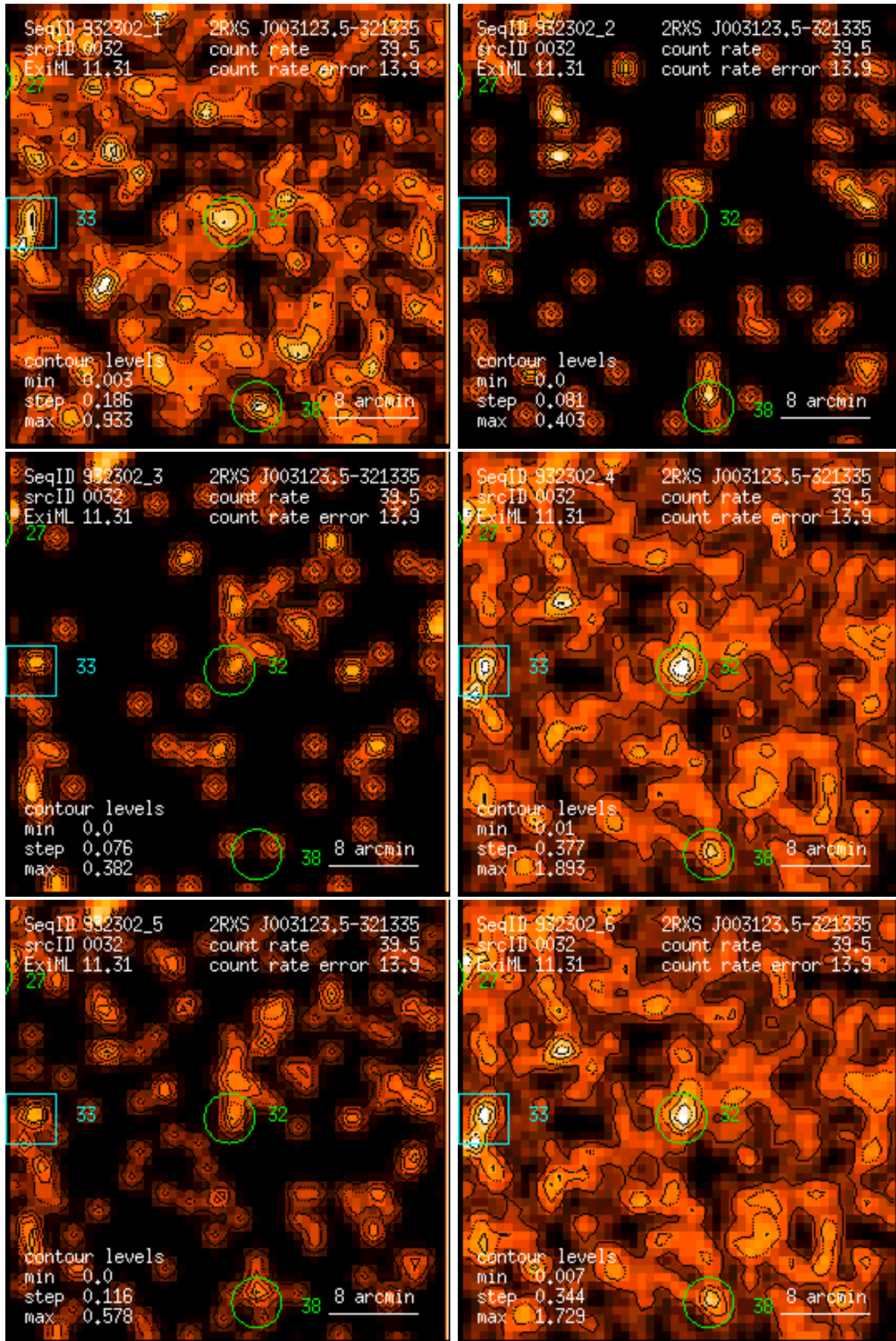
Figure 32: RASS 932302: detection 0032: band rate images, Gaussian filter: (1) PSPC channels 11 – 41, (2) 52 – 90, (3) 91 – 201, (4) 11 – 235, (5) 52 – 201, (6) 11 – 201. Broad band rates in counts/ks. Band rate contour levels in counts/ks/arcmin 2 .
