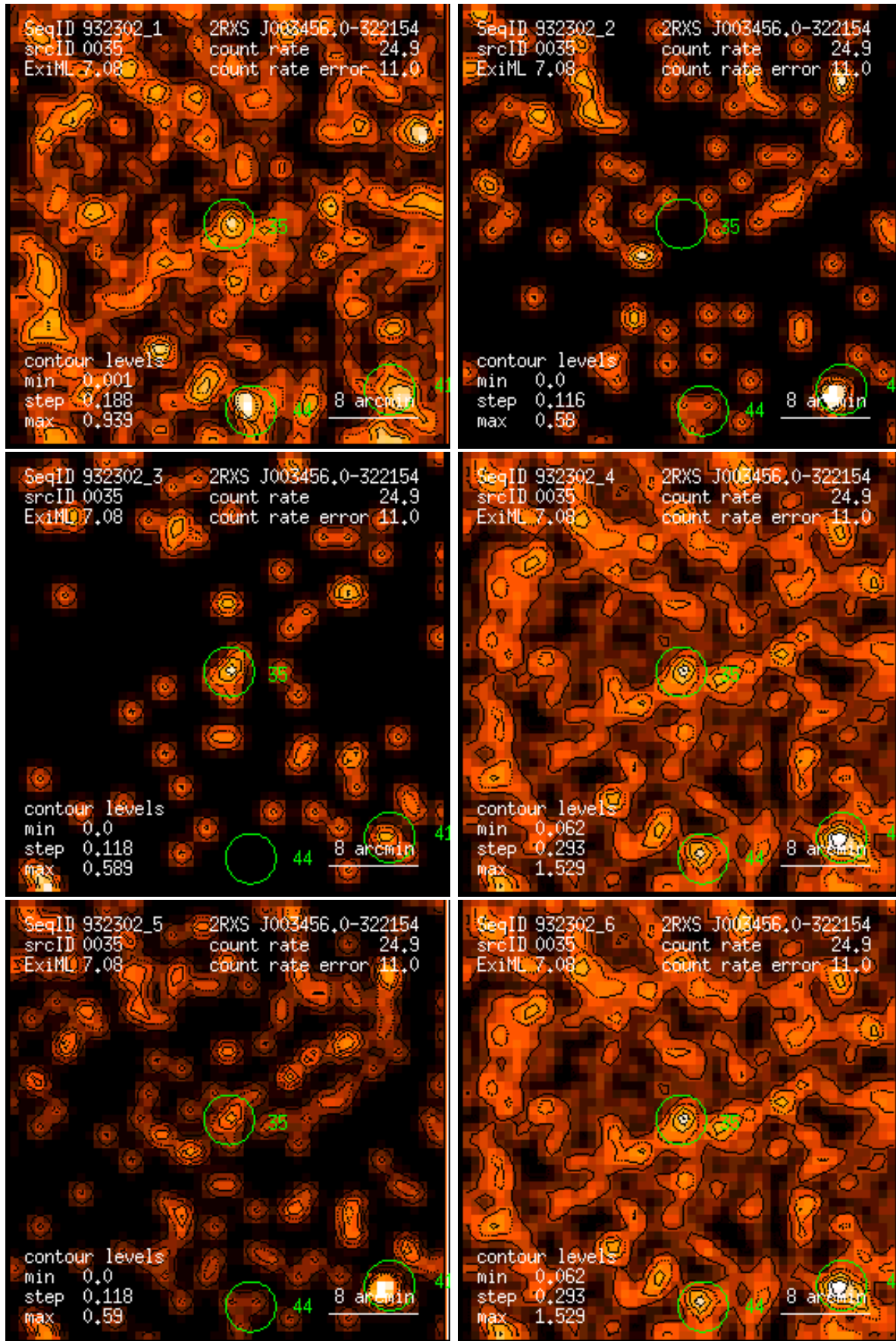
Figure 35: RASS 932302: detection 0035: band rate images, Gaussian filter: (1) PSPC channels 11 – 41, (2) 52 – 90, (3) 91 – 201, (4) 11 – 235, (5) 52 – 201, (6) 11 – 201. Broad band rates in counts/ks. Band rate contour levels in counts/ks/arcmin 2 .
