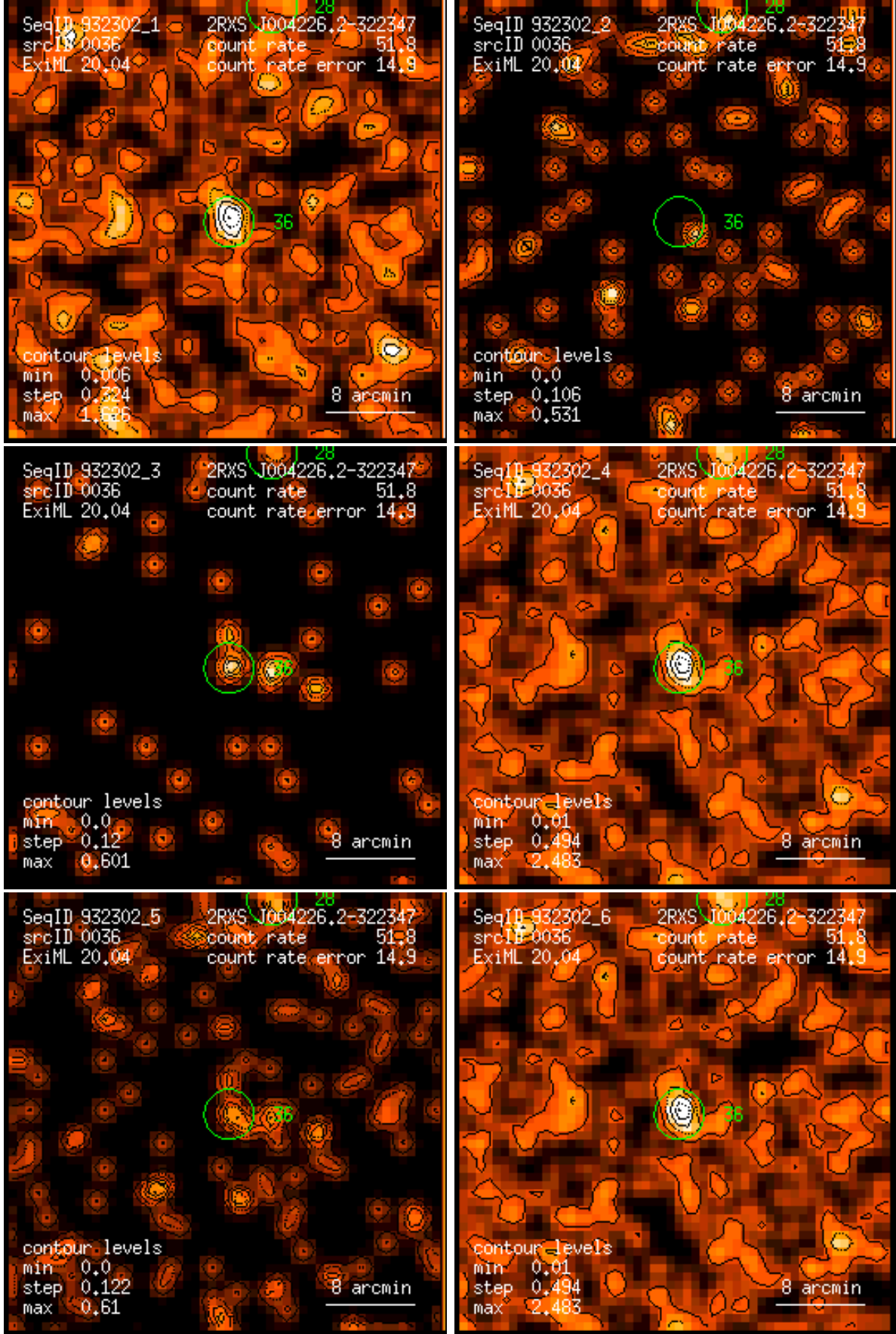
Figure 36: RASS 932302: detection 0036: band rate images, Gaussian filter: (1) PSPC channels 11 – 41, (2) 52 – 90, (3) 91 – 201, (4) 11 – 235, (5) 52 – 201, (6) 11 – 201. Broad band rates in counts/ks. Band rate contour levels in counts/ks/arcmin 2 .
