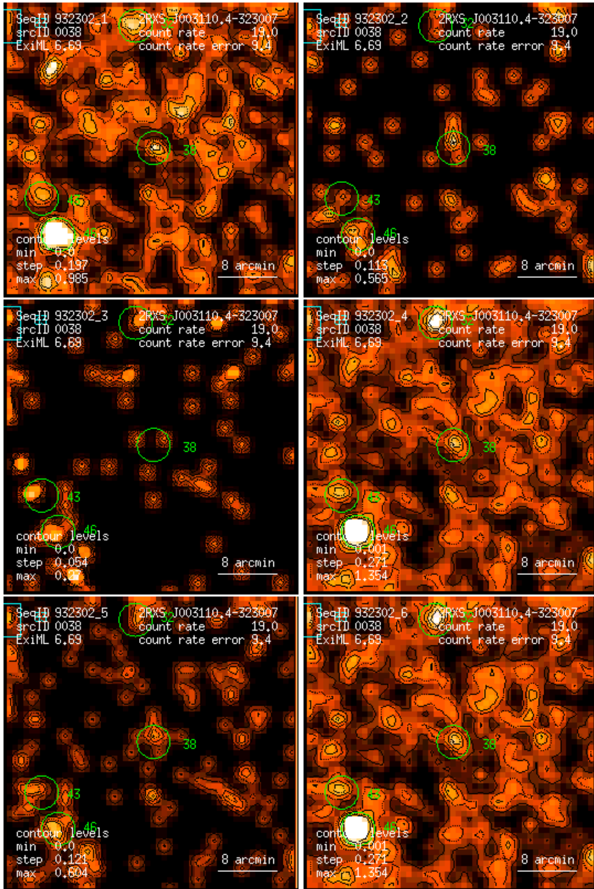
Figure 38: RASS 932302: detection 0038: band rate images, Gaussian filter: (1) PSPC channels 11 – 41, (2) 52 – 90, (3) 91 – 201, (4) 11 – 235, (5) 52 – 201, (6) 11 – 201. Broad band rates in counts/ks. Band rate contour levels in counts/ks/arcmin 2 .
