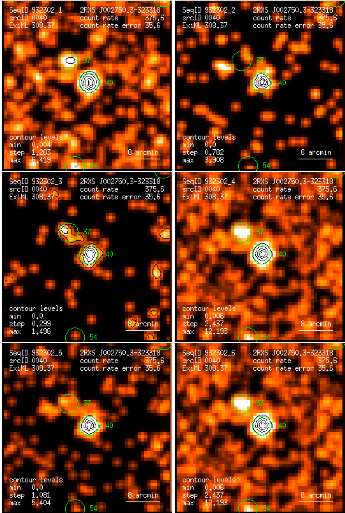
Figure 40: RASS 932302: detection 0040: band rate images, Gaussian filter: (1) PSPC channels 11 – 41, (2) 52 – 90, (3) 91 – 201, (4) 11 – 235, (5) 52 – 201, (6) 11 – 201. Broad band rates in counts/ks. Band rate contour levels in counts/ks/arcmin 2 .
