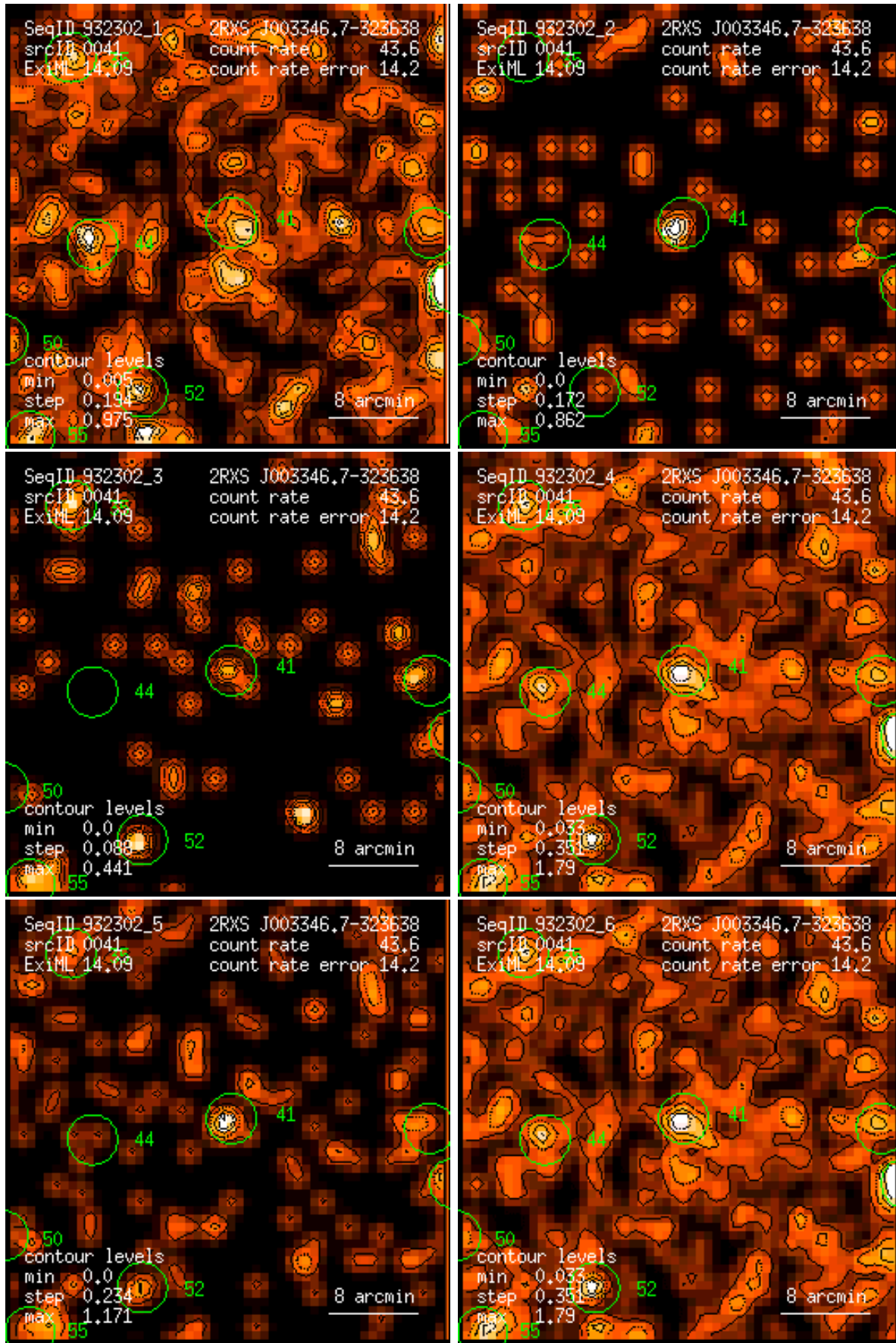
Figure 41: RASS 932302: detection 0041: band rate images, Gaussian filter: (1) PSPC channels 11 – 41, (2) 52 – 90, (3) 91 – 201, (4) 11 – 235, (5) 52 – 201, (6) 11 – 201. Broad band rates in counts/ks. Band rate contour levels in counts/ks/arcmin 2 .
