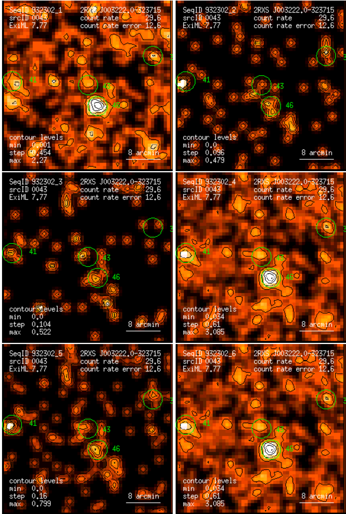
Figure 43: RASS 932302: detection 0043: band rate images, Gaussian filter: (1) PSPC channels 11 – 41, (2) 52 – 90, (3) 91 – 201, (4) 11 – 235, (5) 52 – 201, (6) 11 – 201. Broad band rates in counts/ks. Band rate contour levels in counts/ks/arcmin 2 .
