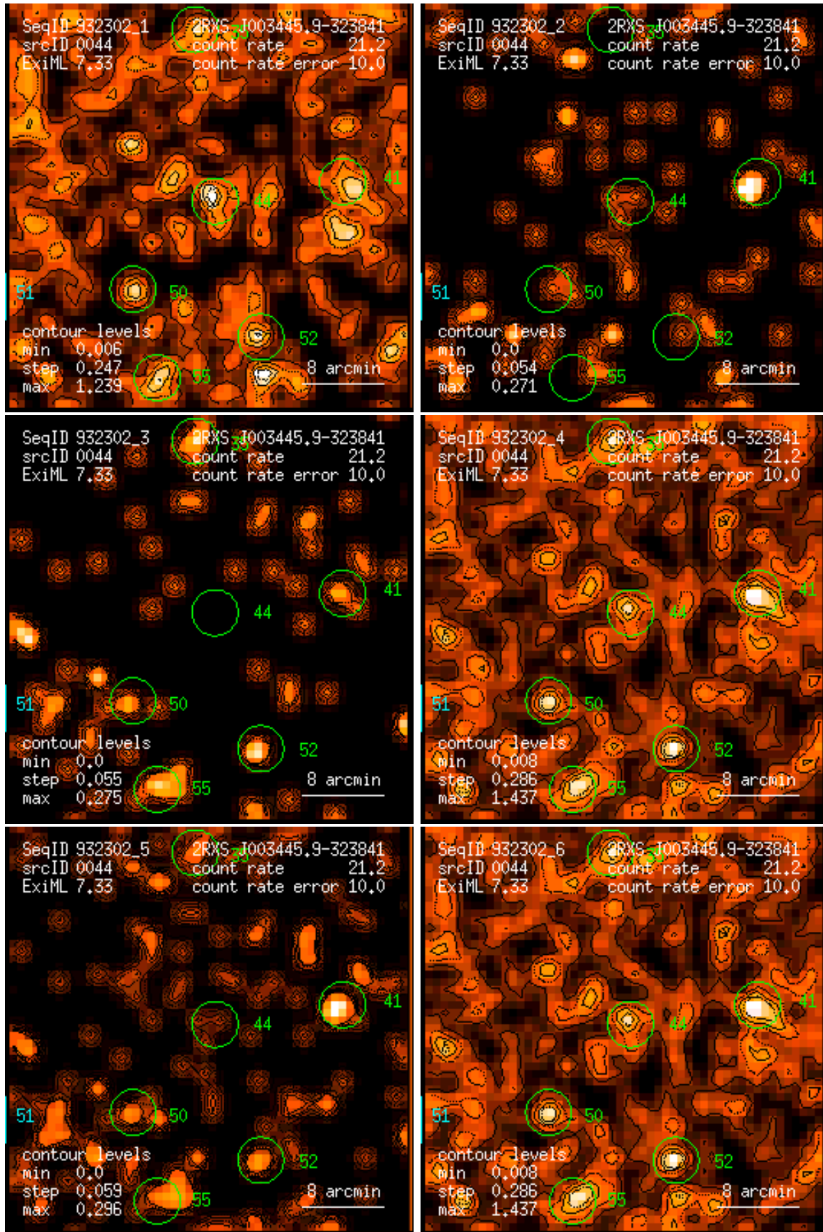
Figure 44: RASS 932302: detection 0044: band rate images, Gaussian filter: (1) PSPC channels 11 – 41, (2) 52 – 90, (3) 91 – 201, (4) 11 – 235, (5) 52 – 201, (6) 11 – 201. Broad band rates in counts/ks. Band rate contour levels in counts/ks/arcmin 2 .
