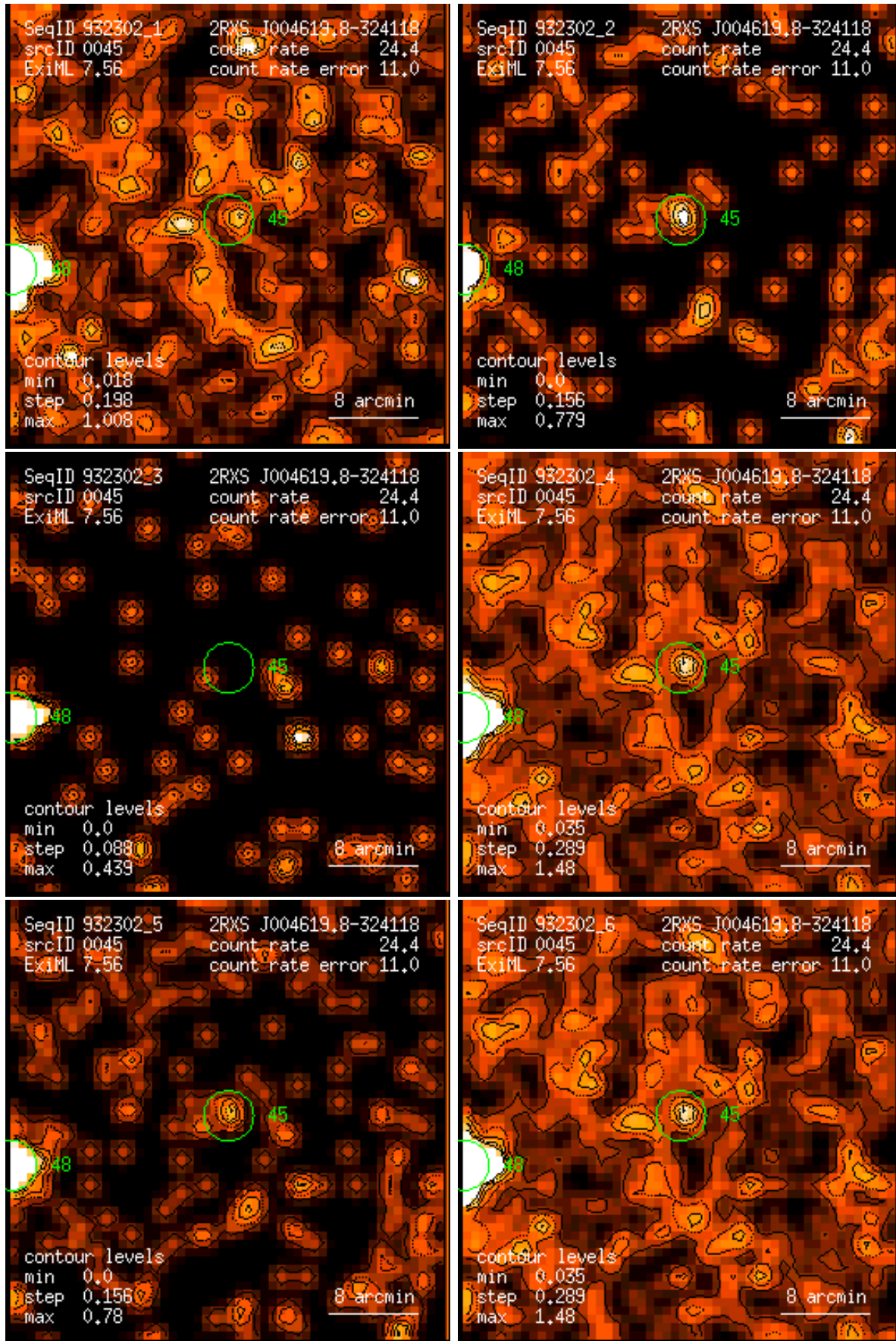
Figure 45: RASS 932302: detection 0045: band rate images, Gaussian filter: (1) PSPC channels 11 – 41, (2) 52 – 90, (3) 91 – 201, (4) 11 – 235, (5) 52 – 201, (6) 11 – 201. Broad band rates in counts/ks. Band rate contour levels in counts/ks/arcmin 2 .
