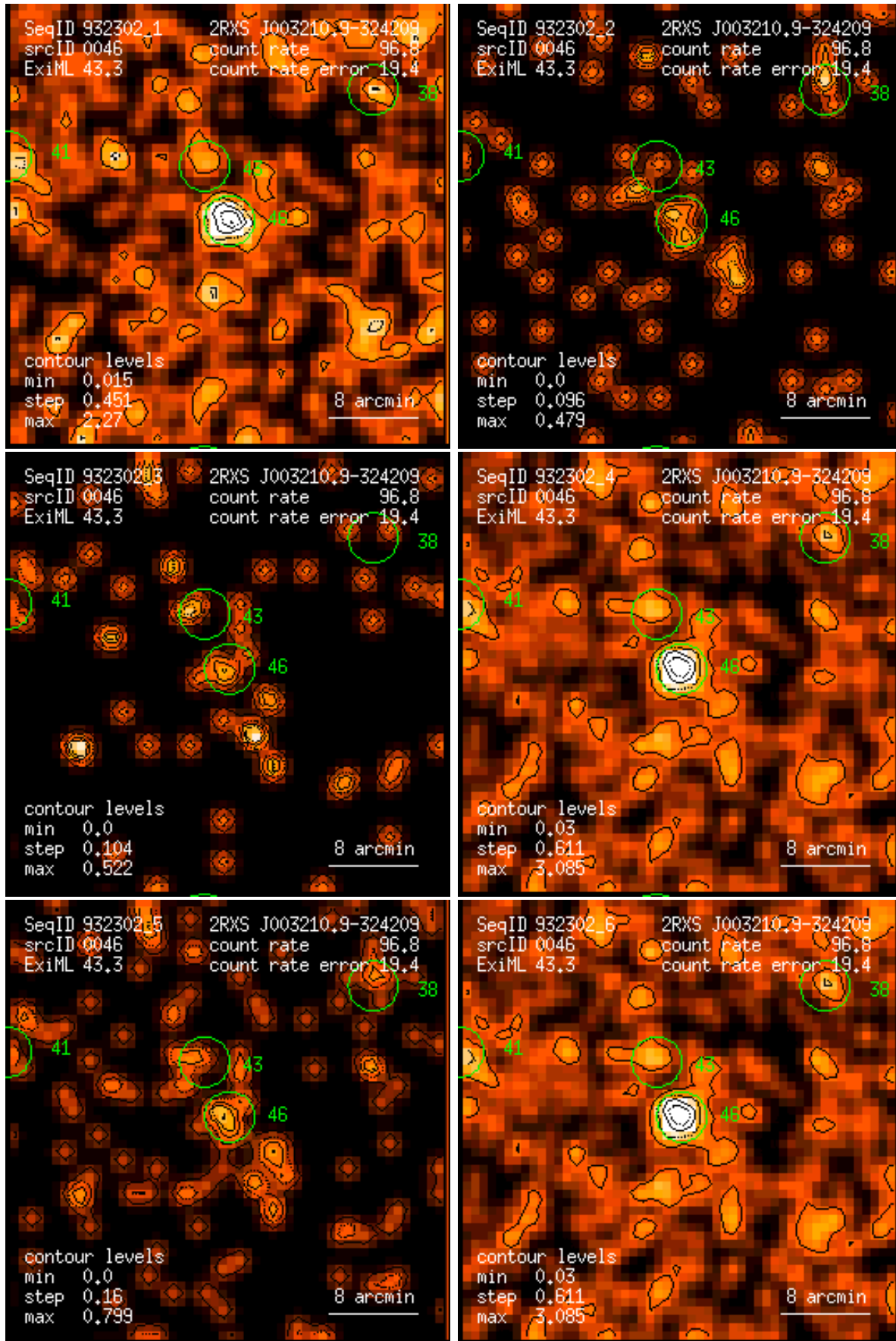
Figure 46: RASS 932302: detection 0046: band rate images, Gaussian filter: (1) PSPC channels 11 – 41, (2) 52 – 90, (3) 91 – 201, (4) 11 – 235, (5) 52 – 201, (6) 11 – 201. Broad band rates in counts/ks. Band rate contour levels in counts/ks/arcmin 2 .
