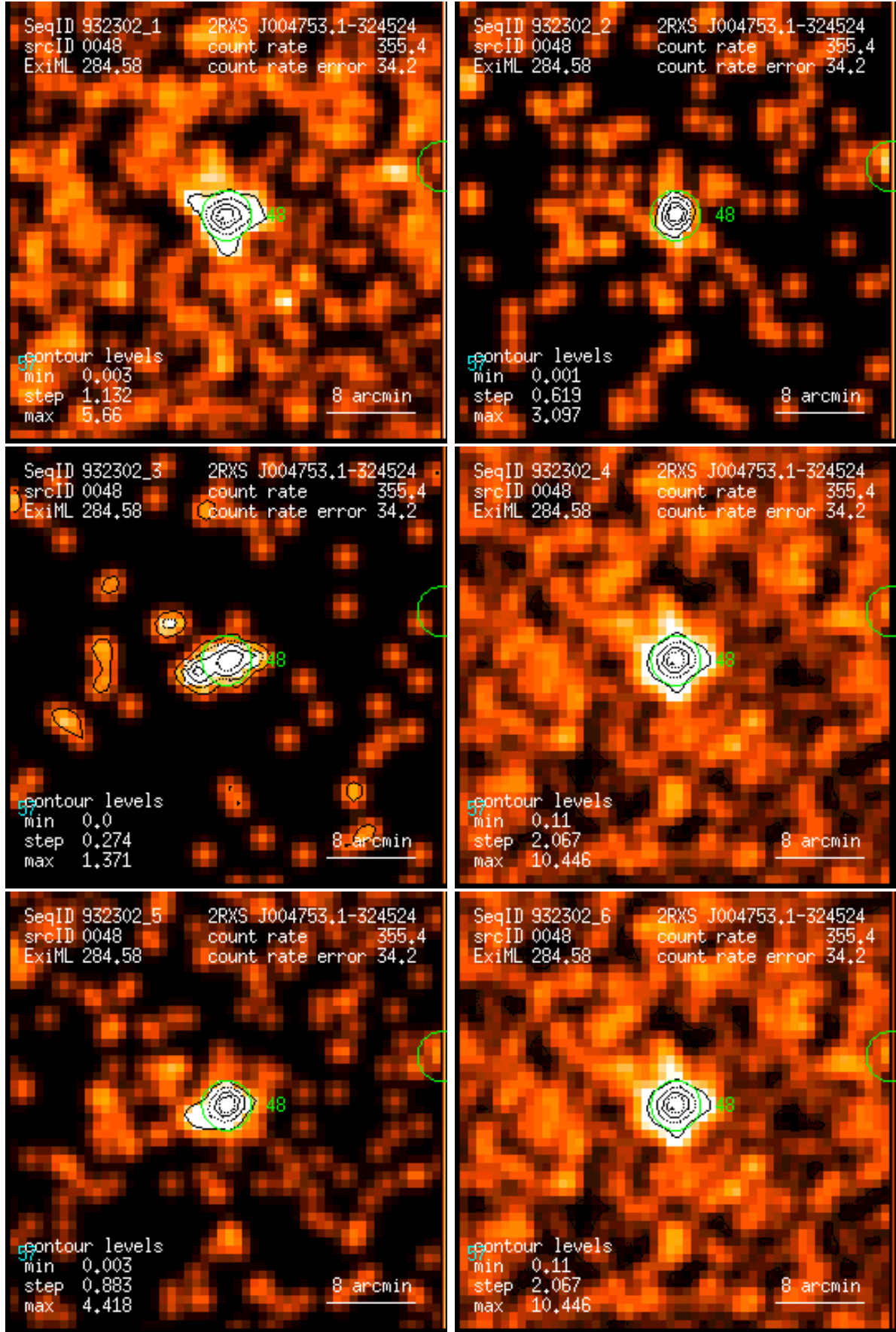
Figure 48: RASS 932302: detection 0048: band rate images, Gaussian filter: (1) PSPC channels 11 – 41, (2) 52 – 90, (3) 91 – 201, (4) 11 – 235, (5) 52 – 201, (6) 11 – 201. Broad band rates in counts/ks. Band rate contour levels in counts/ks/arcmin 2 .
