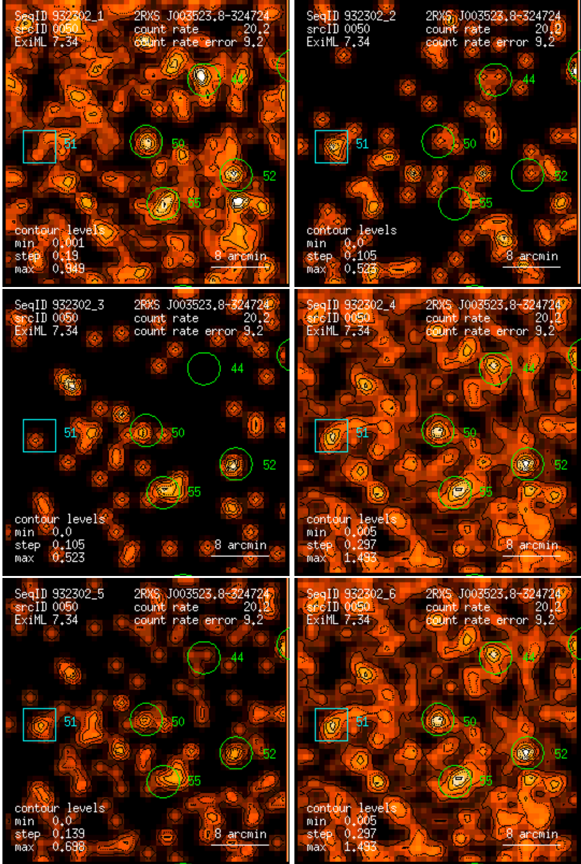
Figure 50: RASS 932302: detection 0050: band rate images, Gaussian filter: (1) PSPC channels 11 – 41, (2) 52 – 90, (3) 91 – 201, (4) 11 – 235, (5) 52 – 201, (6) 11 – 201. Broad band rates in counts/ks. Band rate contour levels in counts/ks/arcmin 2 .
