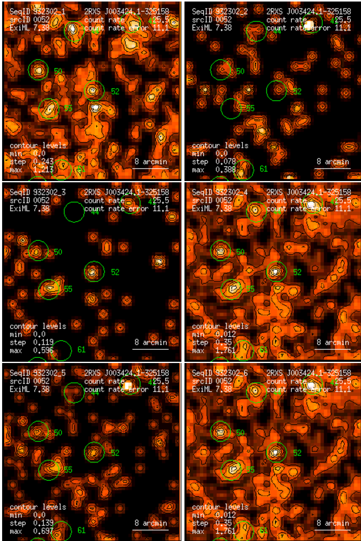
Figure 52: RASS 932302: detection 0052: band rate images, Gaussian filter: (1) PSPC channels 11 – 41, (2) 52 – 90, (3) 91 – 201, (4) 11 – 235, (5) 52 – 201, (6) 11 – 201. Broad band rates in counts/ks. Band rate contour levels in counts/ks/arcmin 2 .
