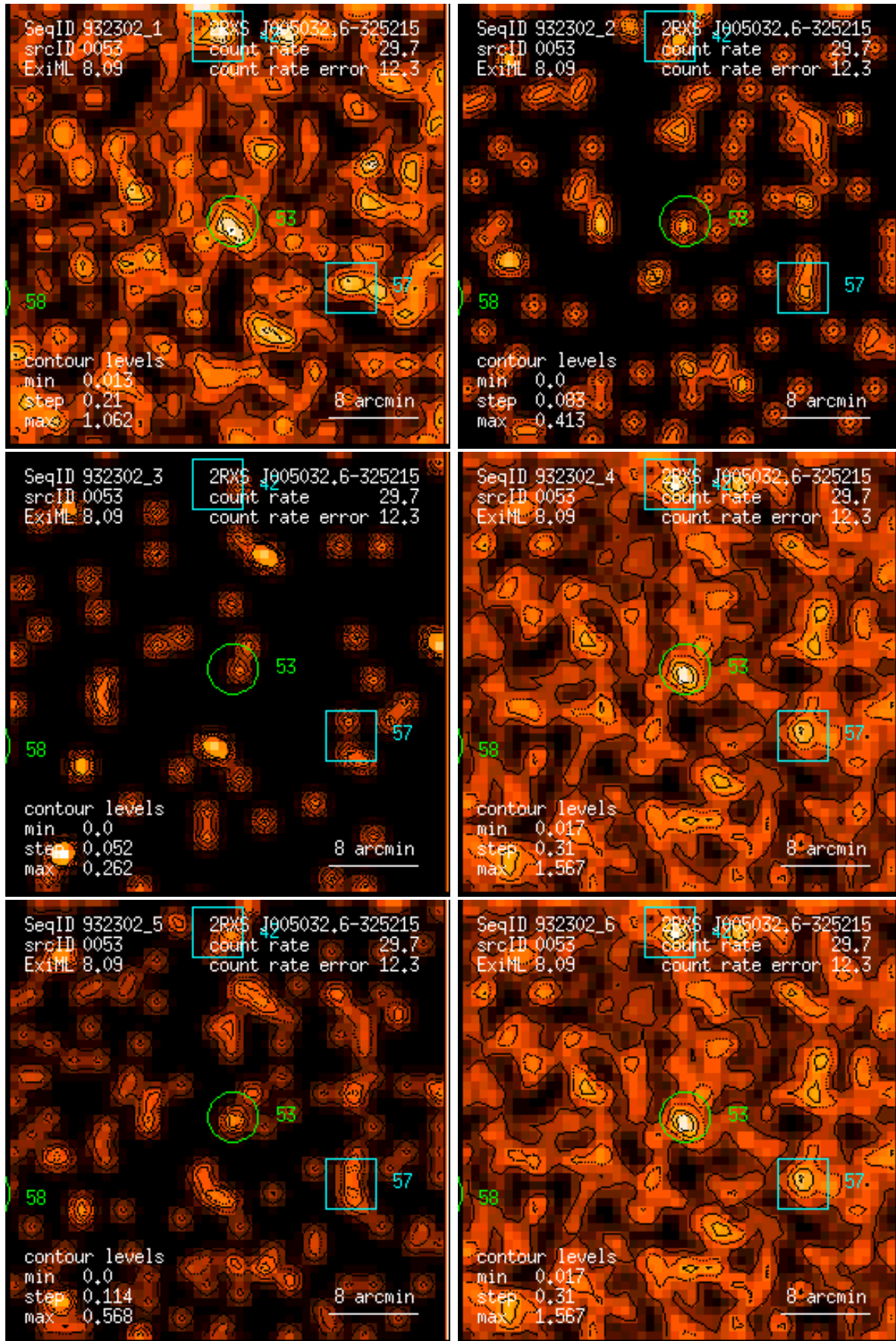
Figure 53: RASS 932302: detection 0053: band rate images, Gaussian filter: (1) PSPC channels 11 – 41, (2) 52 – 90, (3) 91 – 201, (4) 11 – 235, (5) 52 – 201, (6) 11 – 201. Broad band rates in counts/ks. Band rate contour levels in counts/ks/arcmin 2 .
