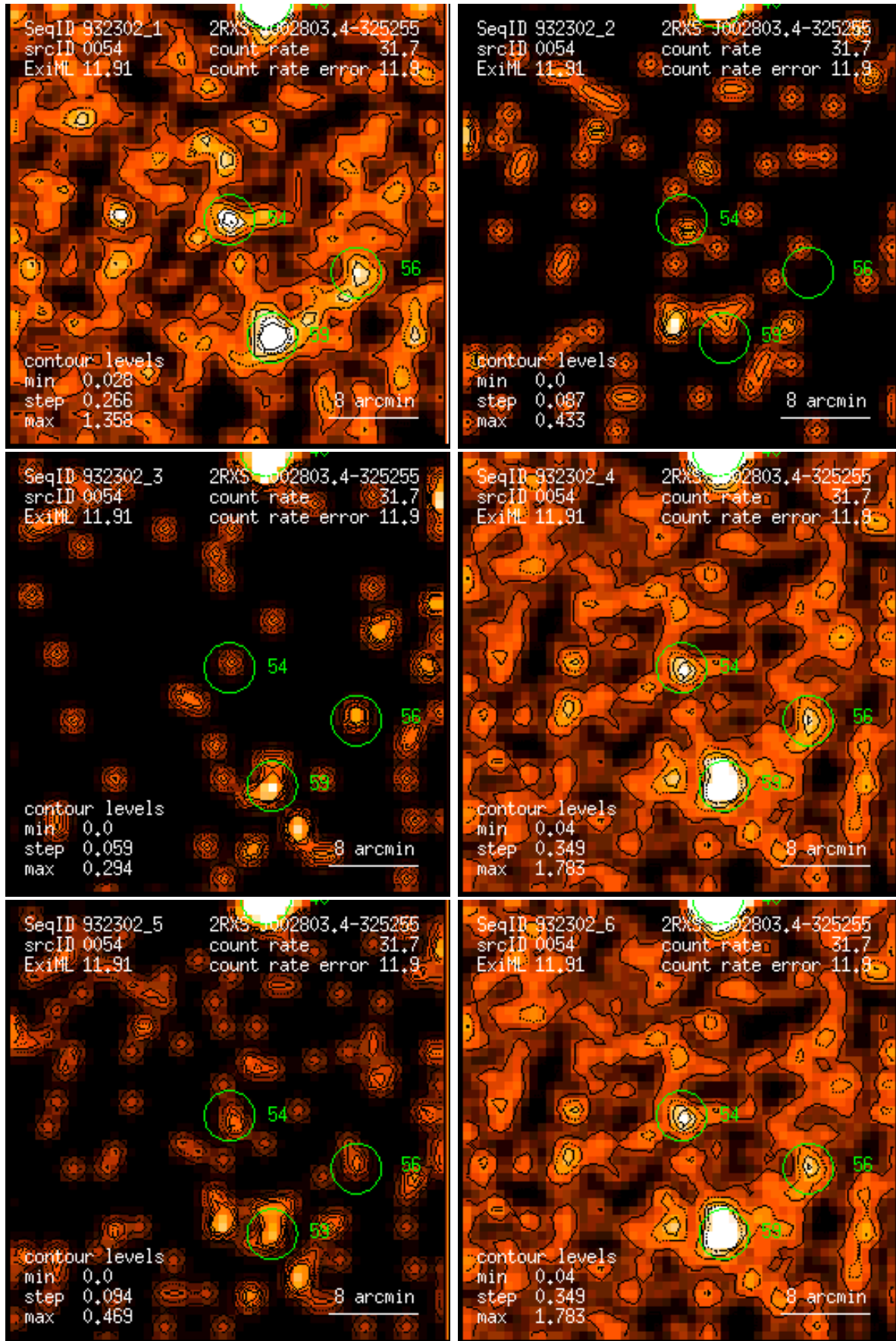
Figure 54: RASS 932302: detection 0054: band rate images, Gaussian filter: (1) PSPC channels 11 – 41, (2) 52 – 90, (3) 91 – 201, (4) 11 – 235, (5) 52 – 201, (6) 11 – 201. Broad band rates in counts/ks. Band rate contour levels in counts/ks/arcmin 2 .
