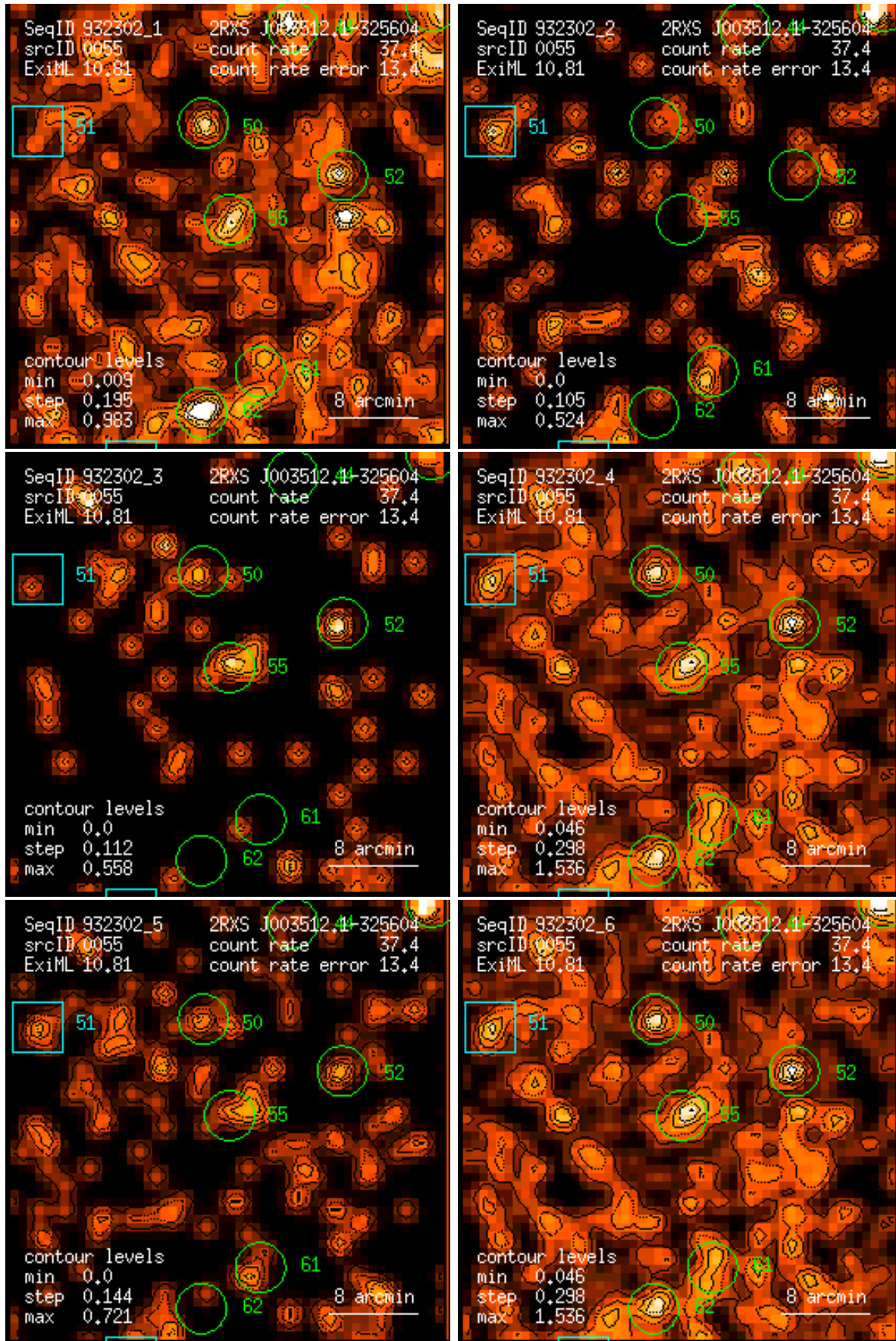
Figure 55: RASS 932302: detection 0055: band rate images, Gaussian filter: (1) PSPC channels 11 – 41, (2) 52 – 90, (3) 91 – 201, (4) 11 – 235, (5) 52 – 201, (6) 11 – 201. Broad band rates in counts/ks. Band rate contour levels in counts/ks/arcmin 2 .
