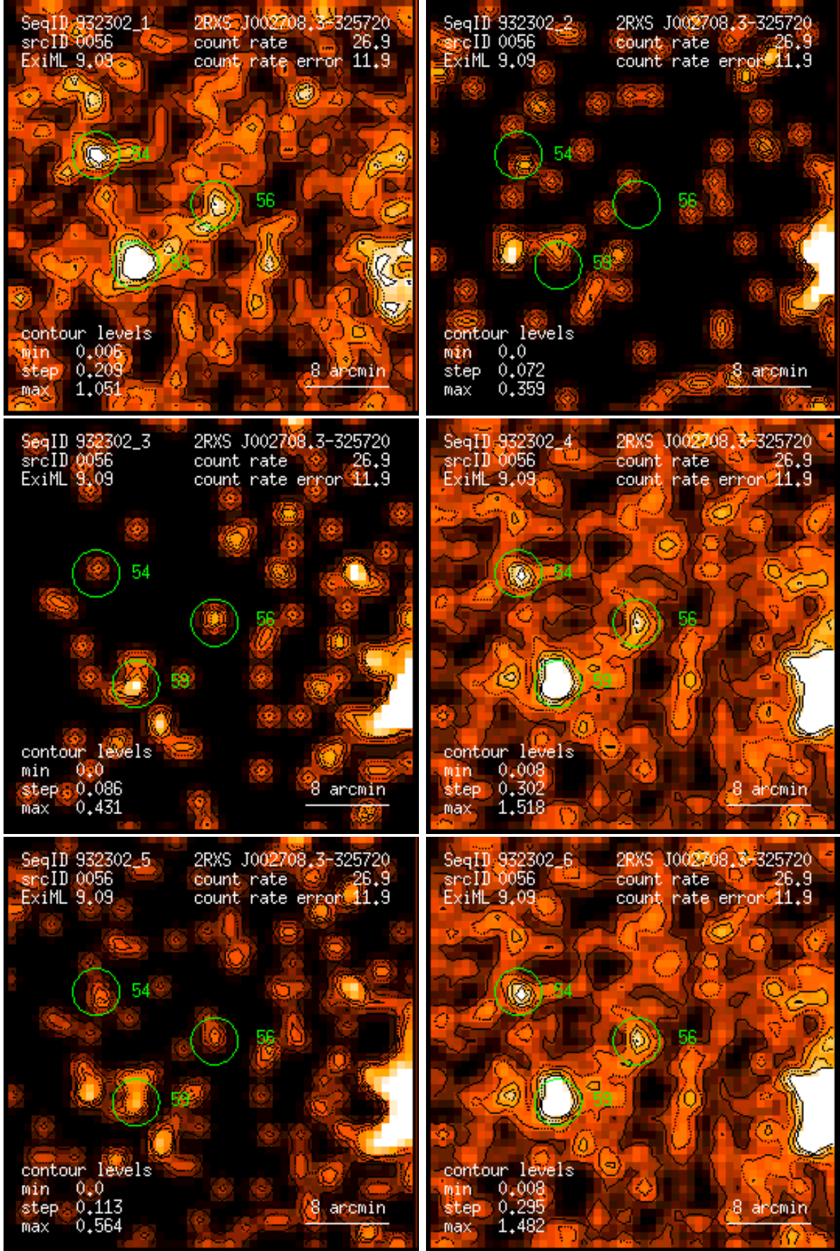
Figure 56: RASS 932302: detection 0056: band rate images, Gaussian filter: (1) PSPC channels 11 – 41, (2) 52 – 90, (3) 91 – 201, (4) 11 – 235, (5) 52 – 201, (6) 11 – 201. Broad band rates in counts/ks. Band rate contour levels in counts/ks/arcmin 2 .
