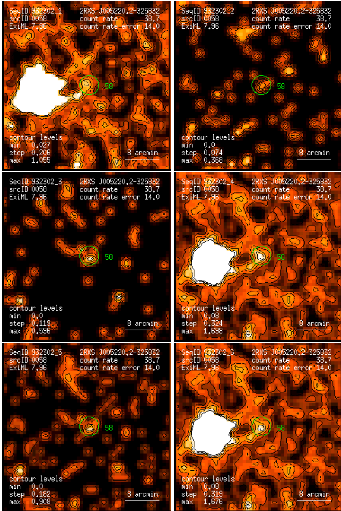
Figure 58: RASS 932302: detection 0058: band rate images, Gaussian filter: (1) PSPC channels 11 – 41, (2) 52 – 90, (3) 91 – 201, (4) 11 – 235, (5) 52 – 201, (6) 11 – 201. Broad band rates in counts/ks. Band rate contour levels in counts/ks/arcmin 2 .
