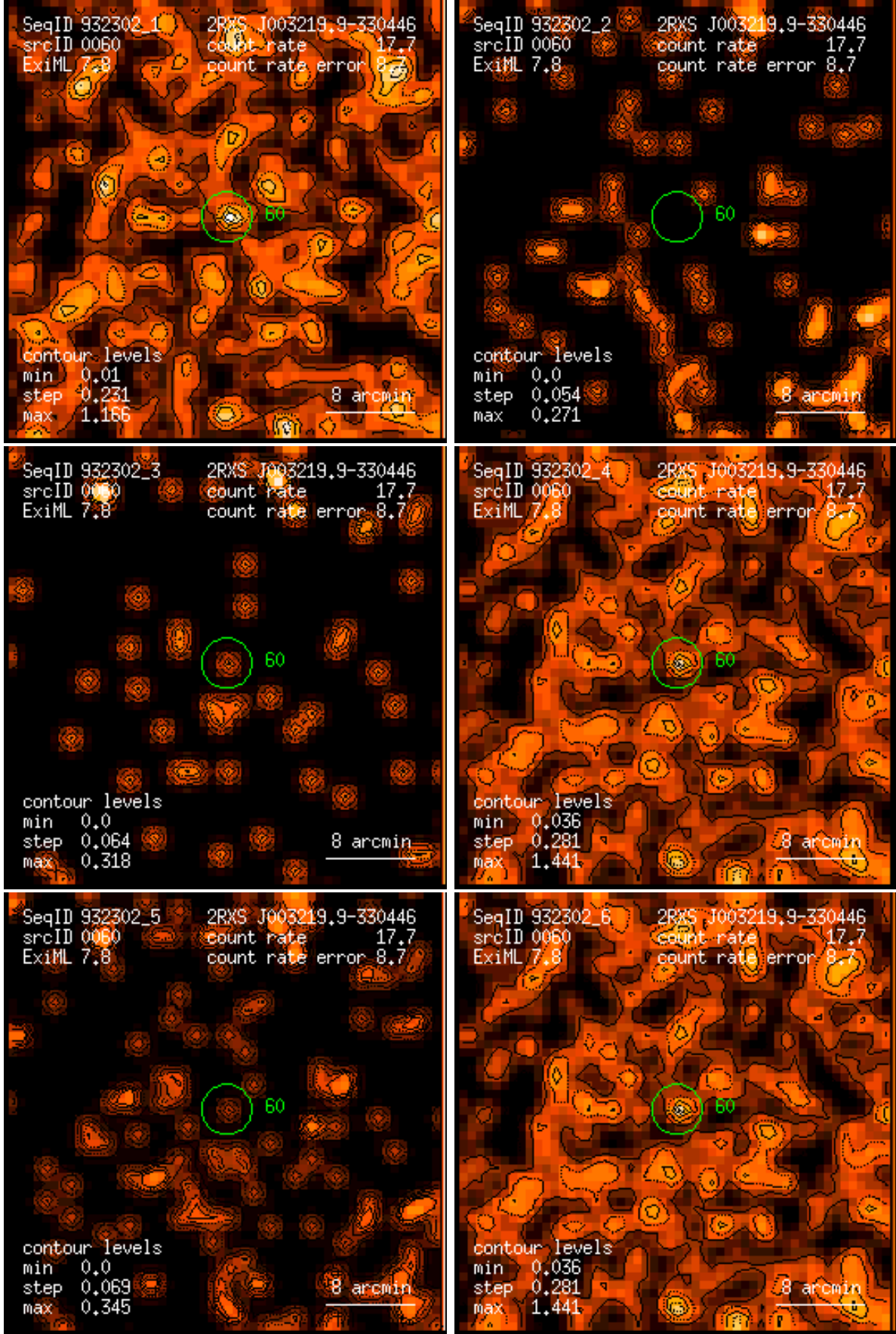
Figure 60: RASS 932302: detection 0060: band rate images, Gaussian filter: (1) PSPC channels 11 – 41, (2) 52 – 90, (3) 91 – 201, (4) 11 – 235, (5) 52 – 201, (6) 11 – 201. Broad band rates in counts/ks. Band rate contour levels in counts/ks/arcmin 2 .
