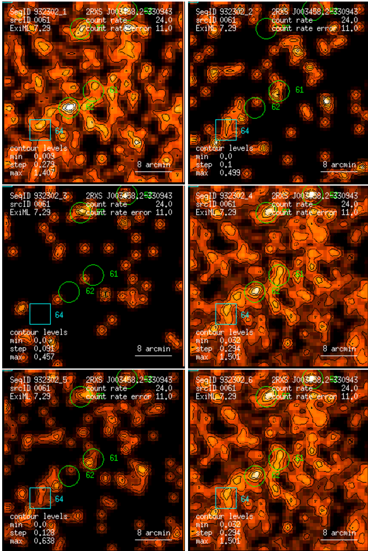
Figure 61: RASS 932302: detection 0061: band rate images, Gaussian filter: (1) PSPC channels 11 – 41, (2) 52 – 90, (3) 91 – 201, (4) 11 – 235, (5) 52 – 201, (6) 11 – 201. Broad band rates in counts/ks. Band rate contour levels in counts/ks/arcmin 2 .
