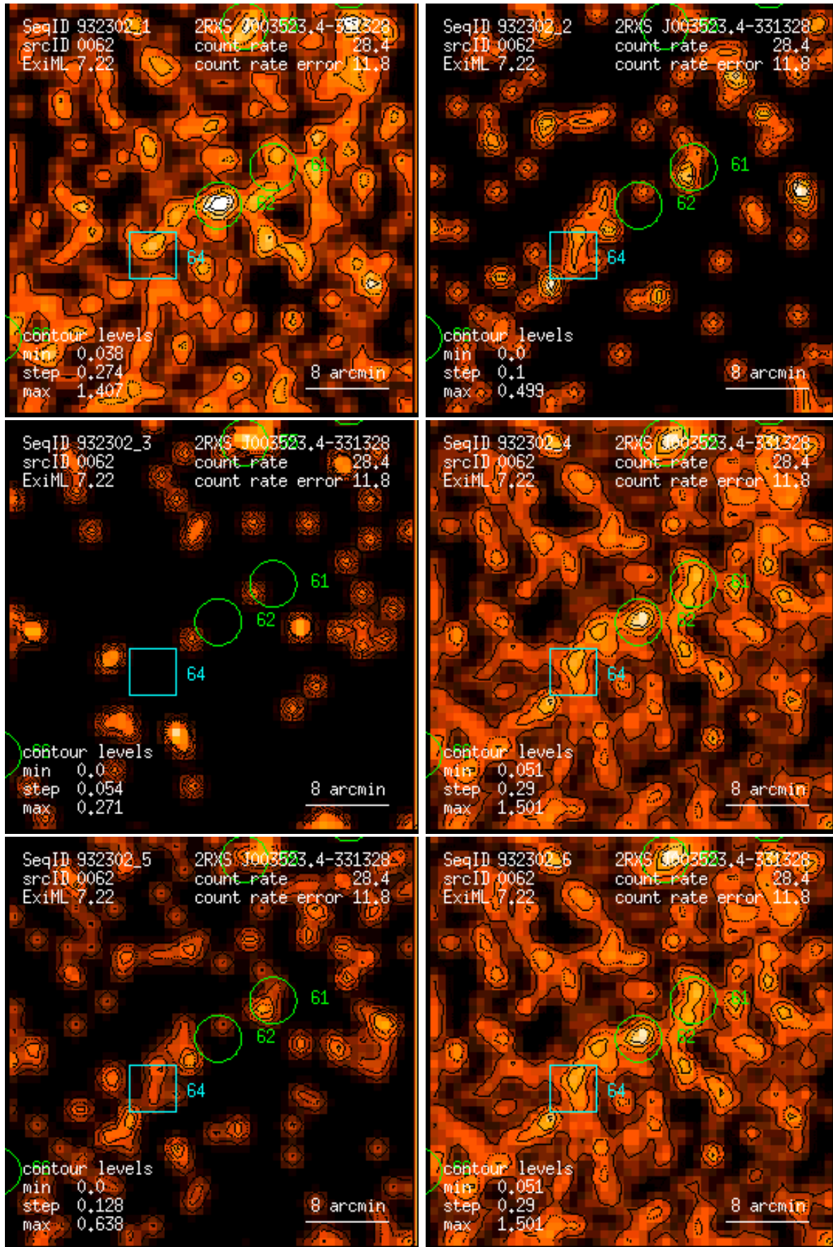
Figure 62: RASS 932302: detection 0062: band rate images, Gaussian filter: (1) PSPC channels 11 – 41, (2) 52 – 90, (3) 91 – 201, (4) 11 – 235, (5) 52 – 201, (6) 11 – 201. Broad band rates in counts/ks. Band rate contour levels in counts/ks/arcmin 2 .
