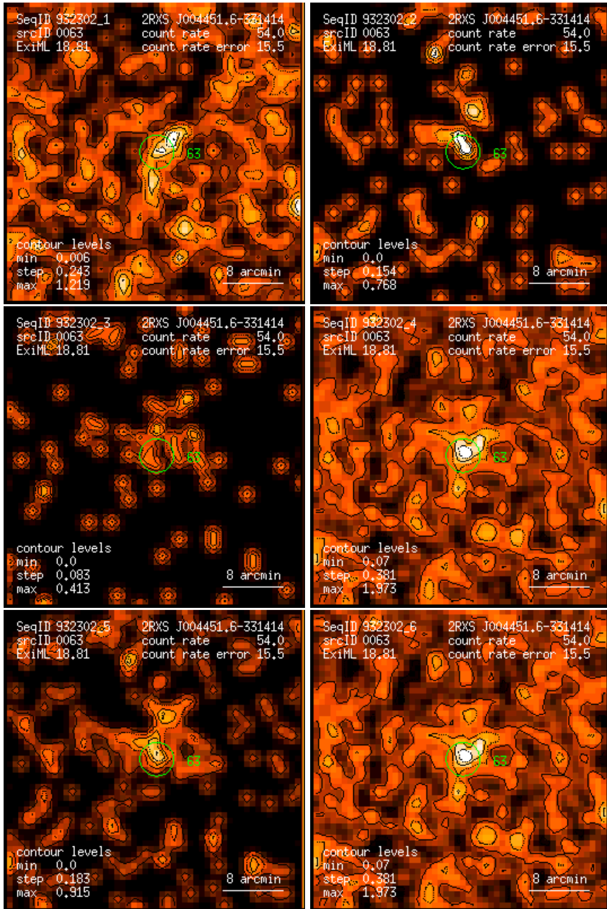
Figure 63: RASS 932302: detection 0063: band rate images, Gaussian filter: (1) PSPC channels 11 – 41, (2) 52 – 90, (3) 91 – 201, (4) 11 – 235, (5) 52 – 201, (6) 11 – 201. Broad band rates in counts/ks. Band rate contour levels in counts/ks/arcmin 2 .
