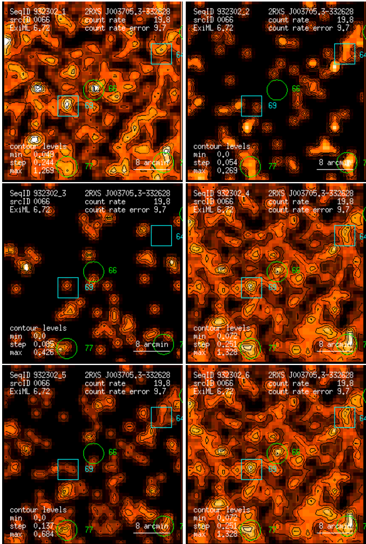
Figure 66: RASS 932302: detection 0066: band rate images, Gaussian filter: (1) PSPC channels 11 – 41, (2) 52 – 90, (3) 91 – 201, (4) 11 – 235, (5) 52 – 201, (6) 11 – 201. Broad band rates in counts/ks. Band rate contour levels in counts/ks/arcmin 2 .
