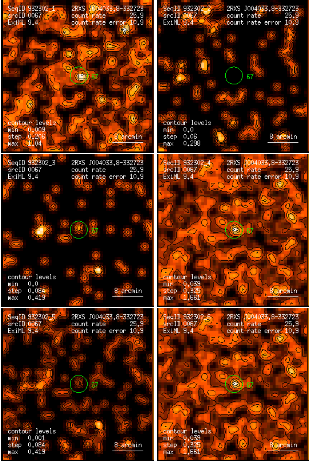
Figure 67: RASS 932302: detection 0067: band rate images, Gaussian filter: (1) PSPC channels 11 – 41, (2) 52 – 90, (3) 91 – 201, (4) 11 – 235, (5) 52 – 201, (6) 11 – 201. Broad band rates in counts/ks. Band rate contour levels in counts/ks/arcmin 2 .
