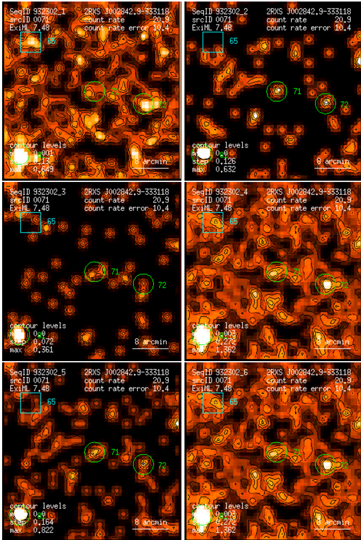
Figure 71: RASS 932302: detection 0071: band rate images, Gaussian filter: (1) PSPC channels 11 – 41, (2) 52 – 90, (3) 91 – 201, (4) 11 – 235, (5) 52 – 201, (6) 11 – 201. Broad band rates in counts/ks. Band rate contour levels in counts/ks/arcmin 2 .
