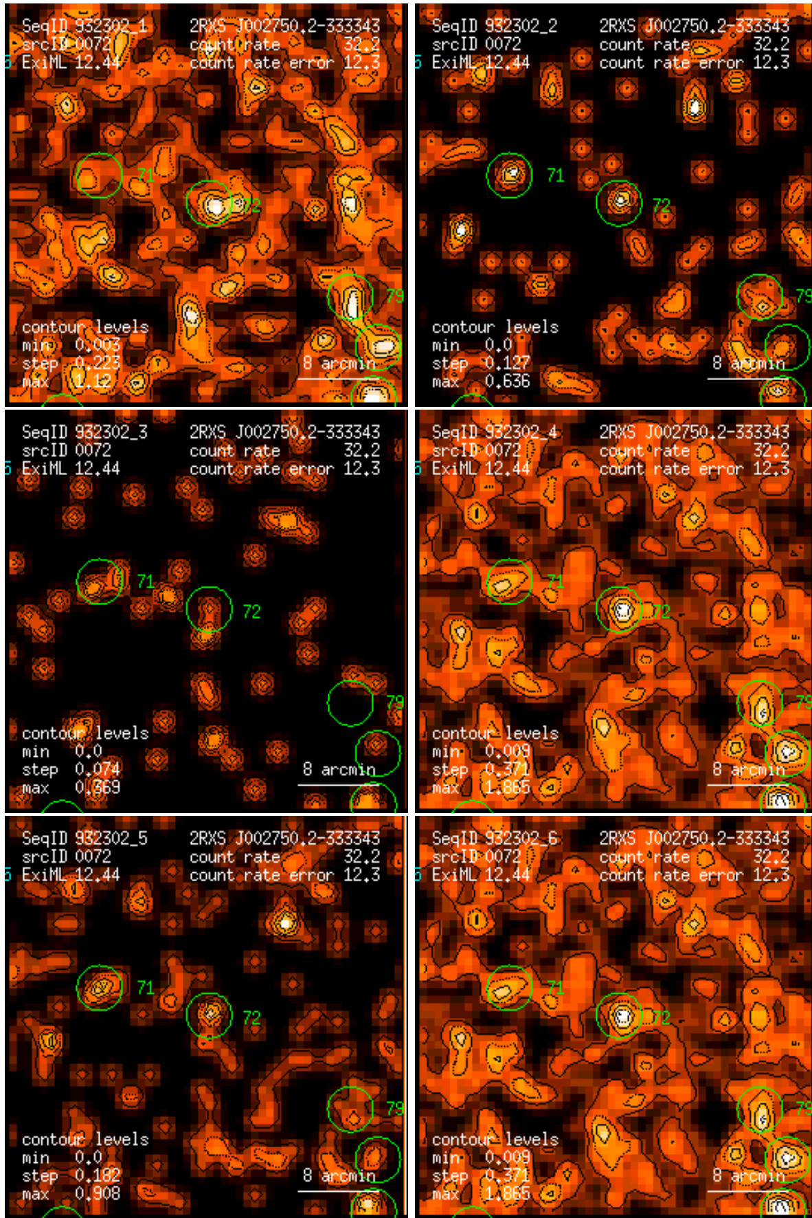
Figure 72: RASS 932302: detection 0072: band rate images, Gaussian filter: (1) PSPC channels 11 – 41, (2) 52 – 90, (3) 91 – 201, (4) 11 – 235, (5) 52 – 201, (6) 11 – 201. Broad band rates in counts/ks. Band rate contour levels in counts/ks/arcmin 2 .
