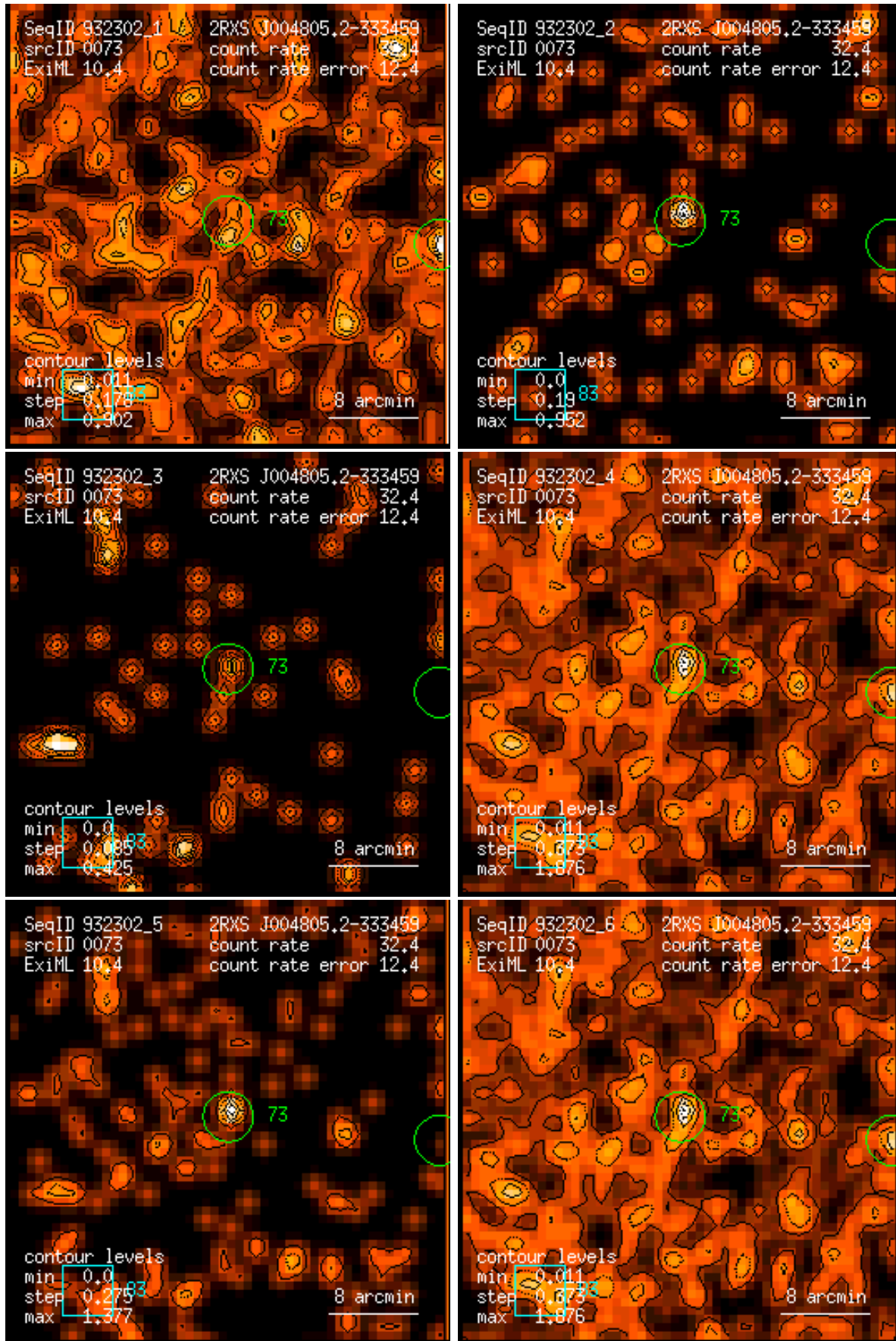
Figure 73: RASS 932302: detection 0073: band rate images, Gaussian filter: (1) PSPC channels 11 – 41, (2) 52 – 90, (3) 91 – 201, (4) 11 – 235, (5) 52 – 201, (6) 11 – 201. Broad band rates in counts/ks. Band rate contour levels in counts/ks/arcmin 2 .
