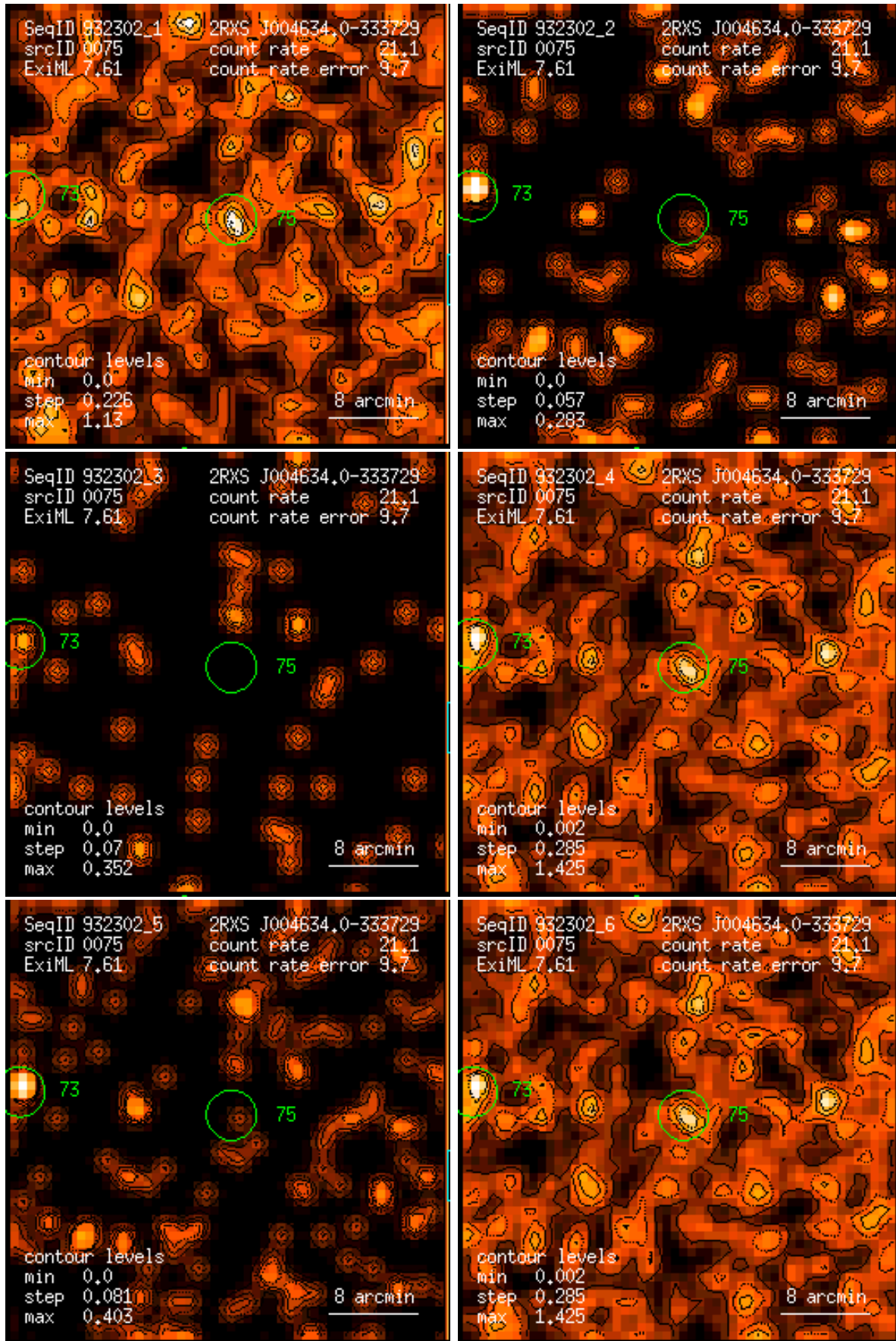
Figure 75: RASS 932302: detection 0075: band rate images, Gaussian filter: (1) PSPC channels 11 – 41, (2) 52 – 90, (3) 91 – 201, (4) 11 – 235, (5) 52 – 201, (6) 11 – 201. Broad band rates in counts/ks. Band rate contour levels in counts/ks/arcmin 2 .
