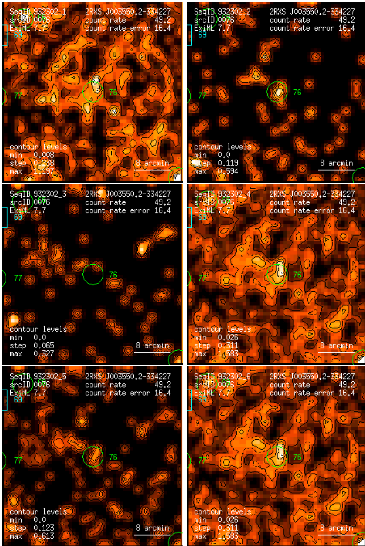
Figure 76: RASS 932302: detection 0076: band rate images, Gaussian filter: (1) PSPC channels 11 – 41, (2) 52 – 90, (3) 91 – 201, (4) 11 – 235, (5) 52 – 201, (6) 11 – 201. Broad band rates in counts/ks. Band rate contour levels in counts/ks/arcmin 2 .
