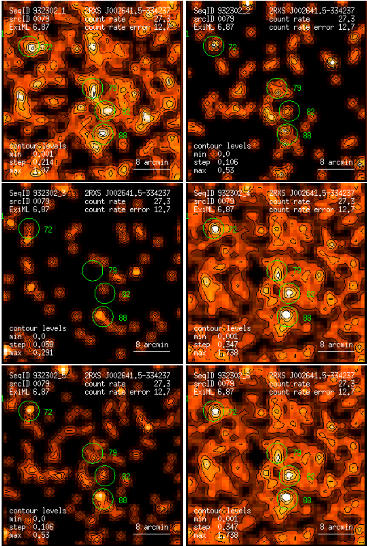
Figure 79: RASS 932302: detection 0079: band rate images, Gaussian filter: (1) PSPC channels 11 – 41, (2) 52 – 90, (3) 91 – 201, (4) 11 – 235, (5) 52 – 201, (6) 11 – 201. Broad band rates in counts/ks. Band rate contour levels in counts/ks/arcmin 2 .
