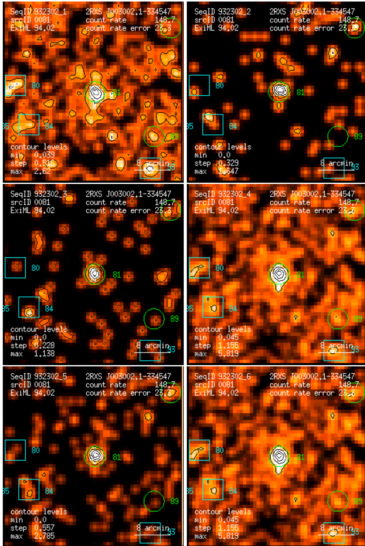
Figure 81: RASS 932302: detection 0081: band rate images, Gaussian filter: (1) PSPC channels 11 – 41, (2) 52 – 90, (3) 91 – 201, (4) 11 – 235, (5) 52 – 201, (6) 11 – 201. Broad band rates in counts/ks. Band rate contour levels in counts/ks/arcmin 2 .
