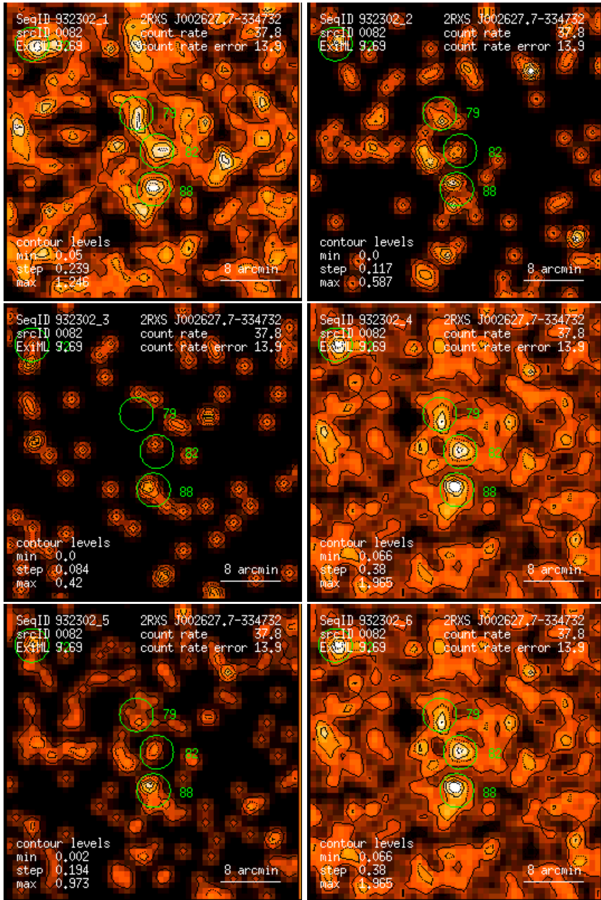
Figure 82: RASS 932302: detection 0082: band rate images, Gaussian filter: (1) PSPC channels 11 – 41, (2) 52 – 90, (3) 91 – 201, (4) 11 – 235, (5) 52 – 201, (6) 11 – 201. Broad band rates in counts/ks. Band rate contour levels in counts/ks/arcmin 2 .
