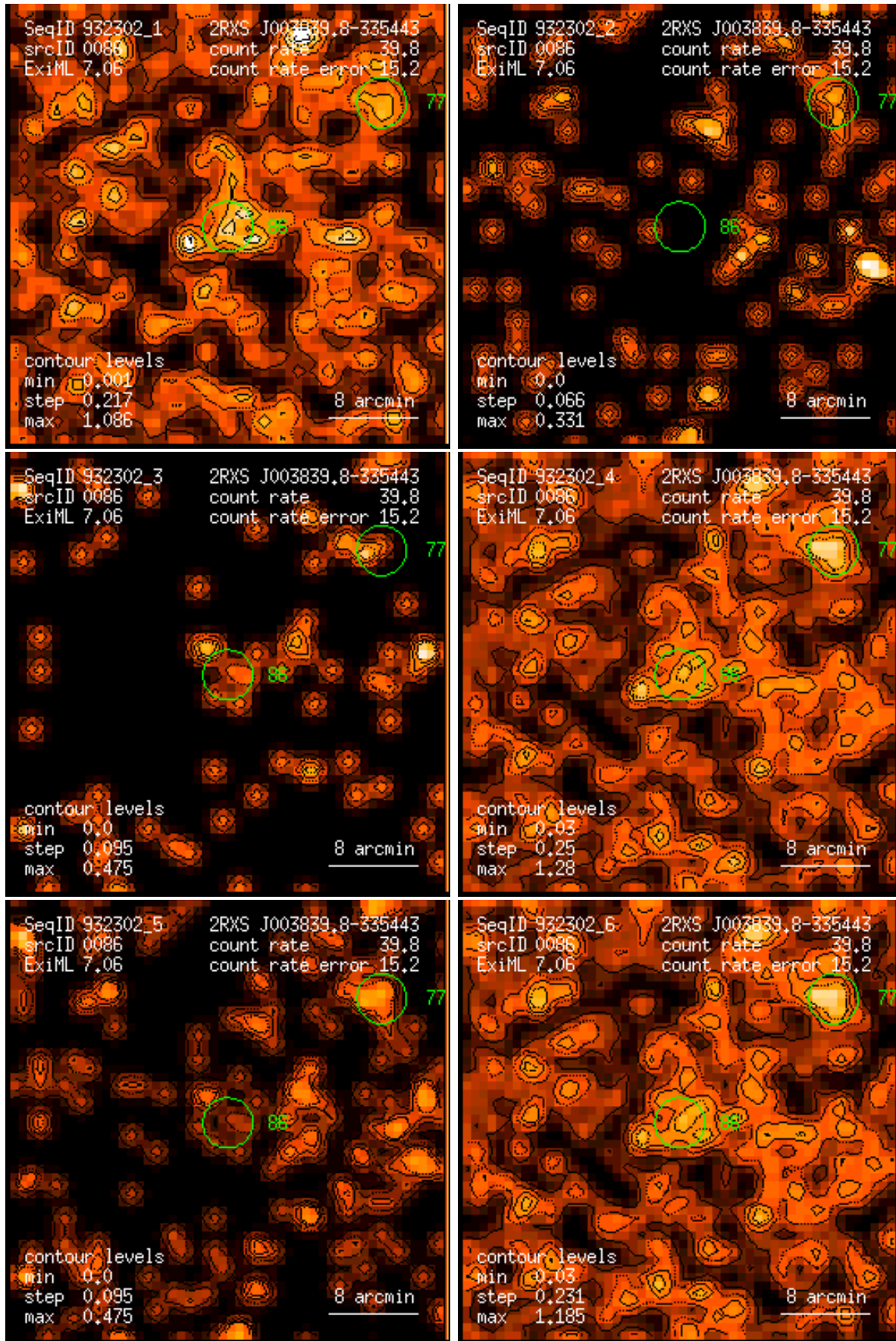
Figure 86: RASS 932302: detection 0086: band rate images, Gaussian filter: (1) PSPC channels 11 – 41, (2) 52 – 90, (3) 91 – 201, (4) 11 – 235, (5) 52 – 201, (6) 11 – 201. Broad band rates in counts/ks. Band rate contour levels in counts/ks/arcmin 2 .
