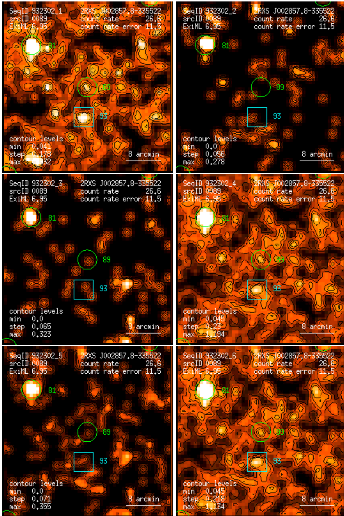
Figure 89: RASS 932302: detection 0089: band rate images, Gaussian filter: (1) PSPC channels 11 – 41, (2) 52 – 90, (3) 91 – 201, (4) 11 – 235, (5) 52 – 201, (6) 11 – 201. Broad band rates in counts/ks. Band rate contour levels in counts/ks/arcmin 2 .
