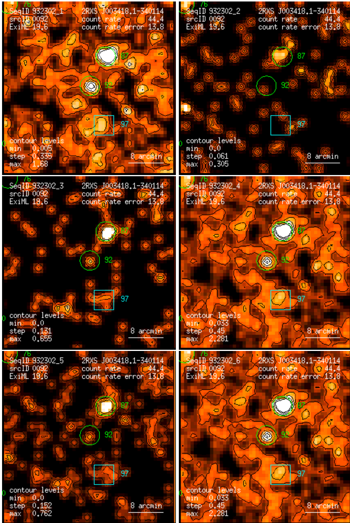
Figure 92: RASS 932302: detection 0092: band rate images, Gaussian filter: (1) PSPC channels 11 – 41, (2) 52 – 90, (3) 91 – 201, (4) 11 – 235, (5) 52 – 201, (6) 11 – 201. Broad band rates in counts/ks. Band rate contour levels in counts/ks/arcmin 2 .
