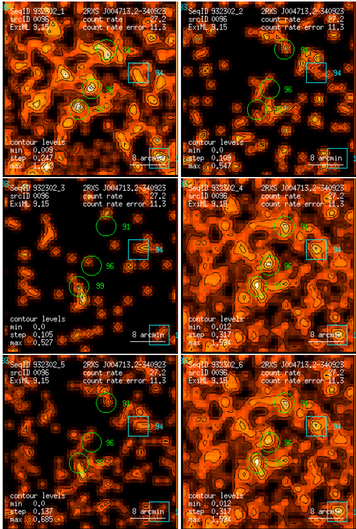
Figure 96: RASS 932302: detection 0096: band rate images, Gaussian filter: (1) PSPC channels 11 – 41, (2) 52 – 90, (3) 91 – 201, (4) 11 – 235, (5) 52 – 201, (6) 11 – 201. Broad band rates in counts/ks. Band rate contour levels in counts/ks/arcmin 2 .
