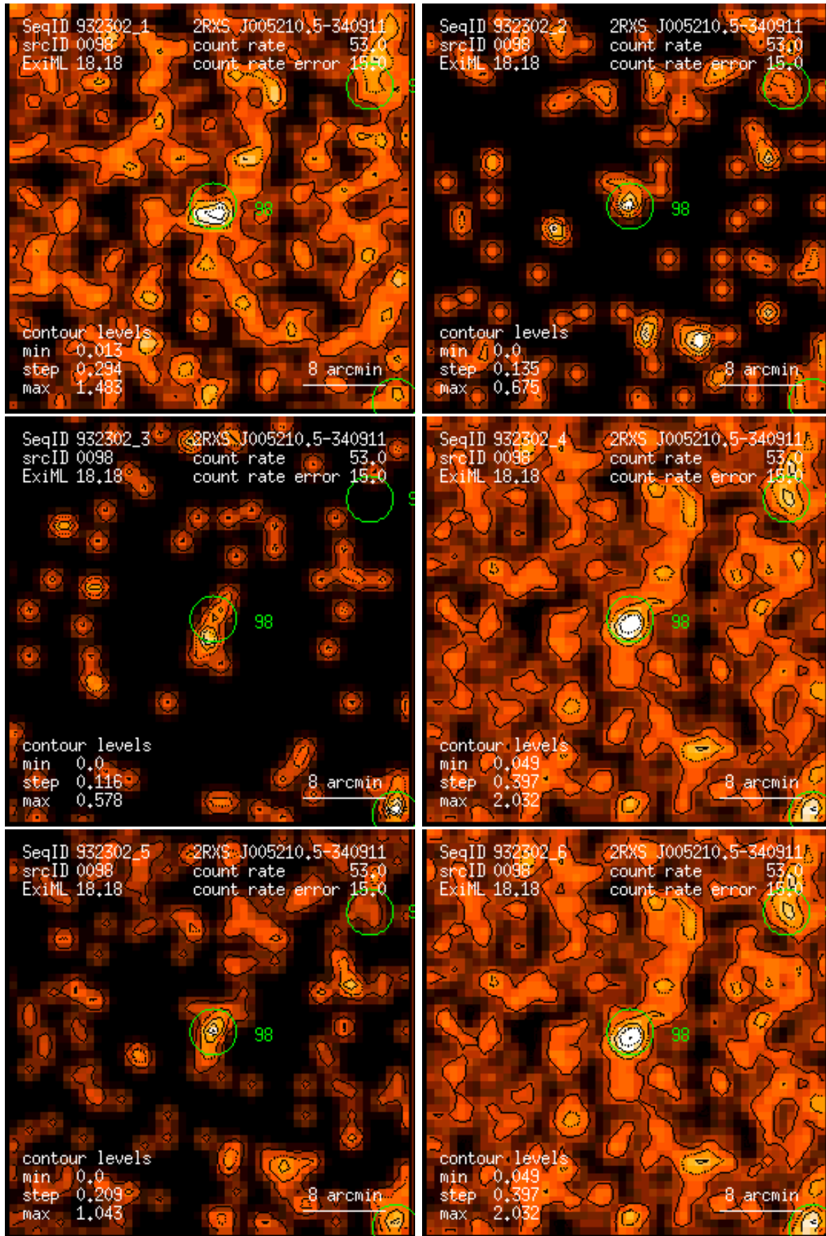
Figure 98: RASS 932302: detection 0098: band rate images, Gaussian filter: (1) PSPC channels 11 – 41, (2) 52 – 90, (3) 91 – 201, (4) 11 – 235, (5) 52 – 201, (6) 11 – 201. Broad band rates in counts/ks. Band rate contour levels in counts/ks/arcmin 2 .
