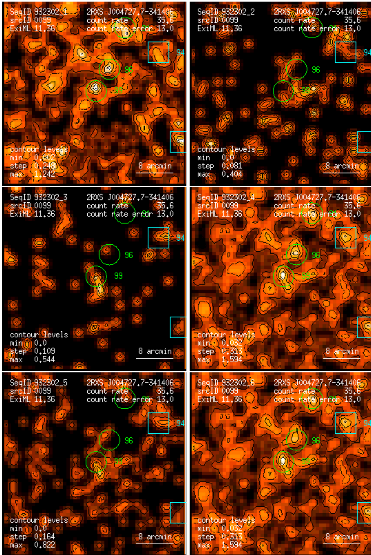
Figure 99: RASS 932302: detection 0099: band rate images, Gaussian filter: (1) PSPC channels 11 – 41, (2) 52 – 90, (3) 91 – 201, (4) 11 – 235, (5) 52 – 201, (6) 11 – 201. Broad band rates in counts/ks. Band rate contour levels in counts/ks/arcmin 2 .
