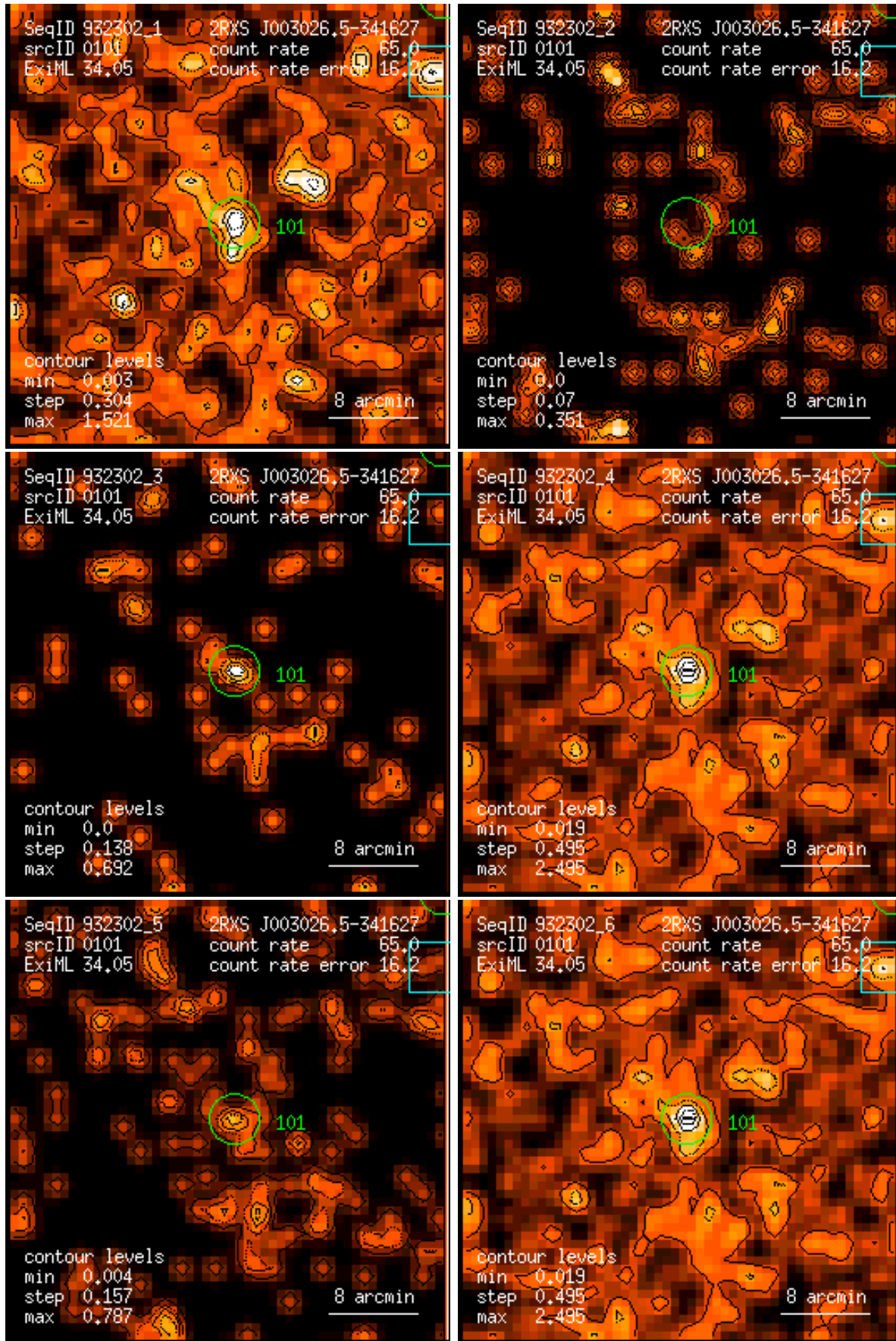
Figure 101: RASS 932302: detection 0101: band rate images, Gaussian filter: (1) PSPC channels 11 – 41, (2) 52 – 90, (3) 91 – 201, (4) 11 – 235, (5) 52 – 201, (6) 11 – 201. Broad band rates in counts/ks. Band rate contour levels in counts/ks/arcmin 2 .
